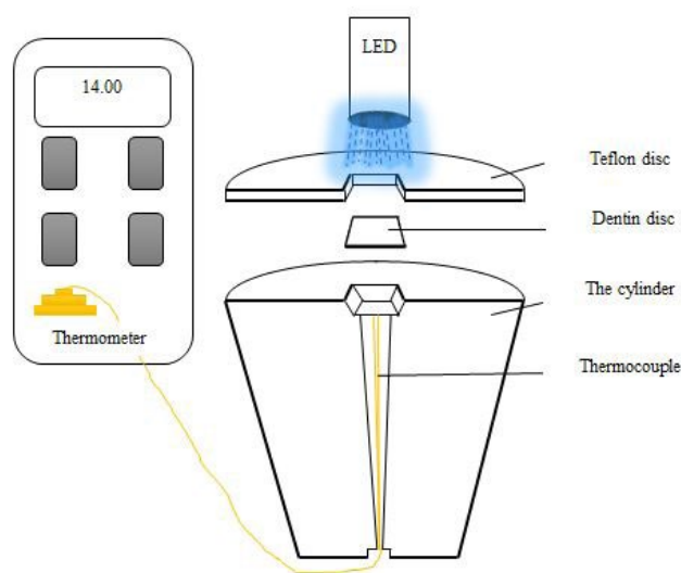
Figure 1: Temperature Test Apparatus
