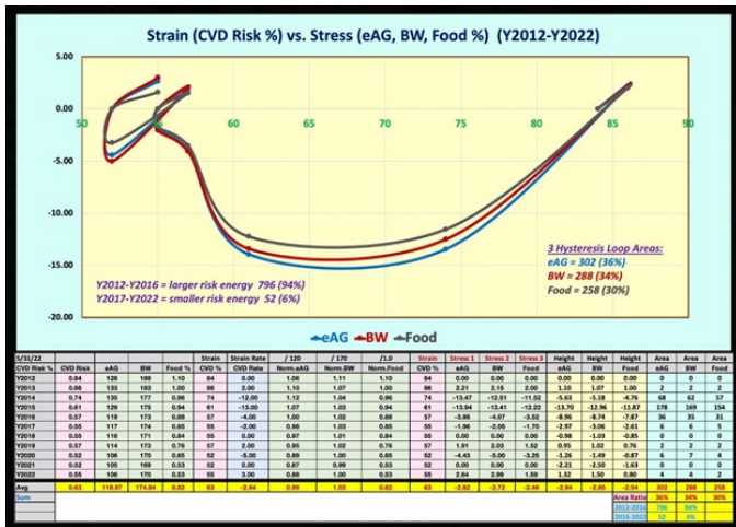
Figure 2: Space-domain VGT stress-strain analysis results of CVD risk, eAG, BW, and food portion during 11 years
