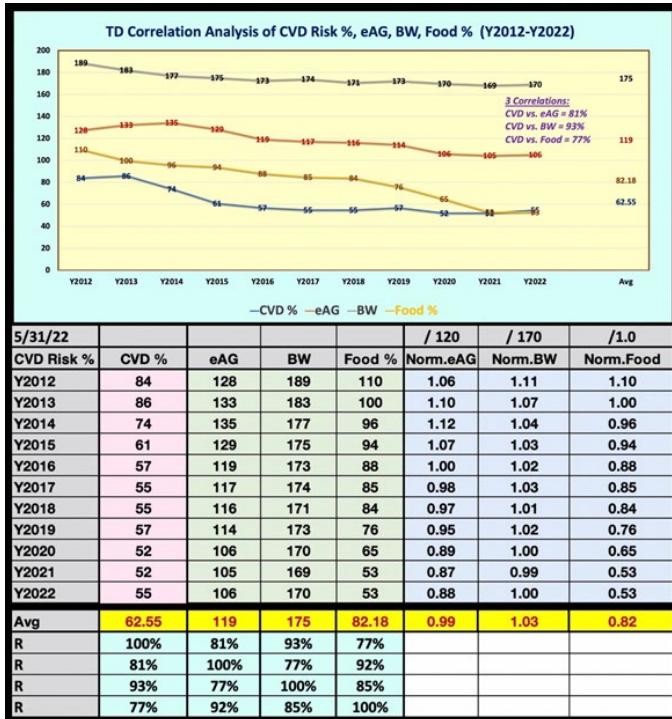
Figure 1: Time-domain analysis results of CVD risk, eAG, BW, and food portion with multiple correlations during 11 years
