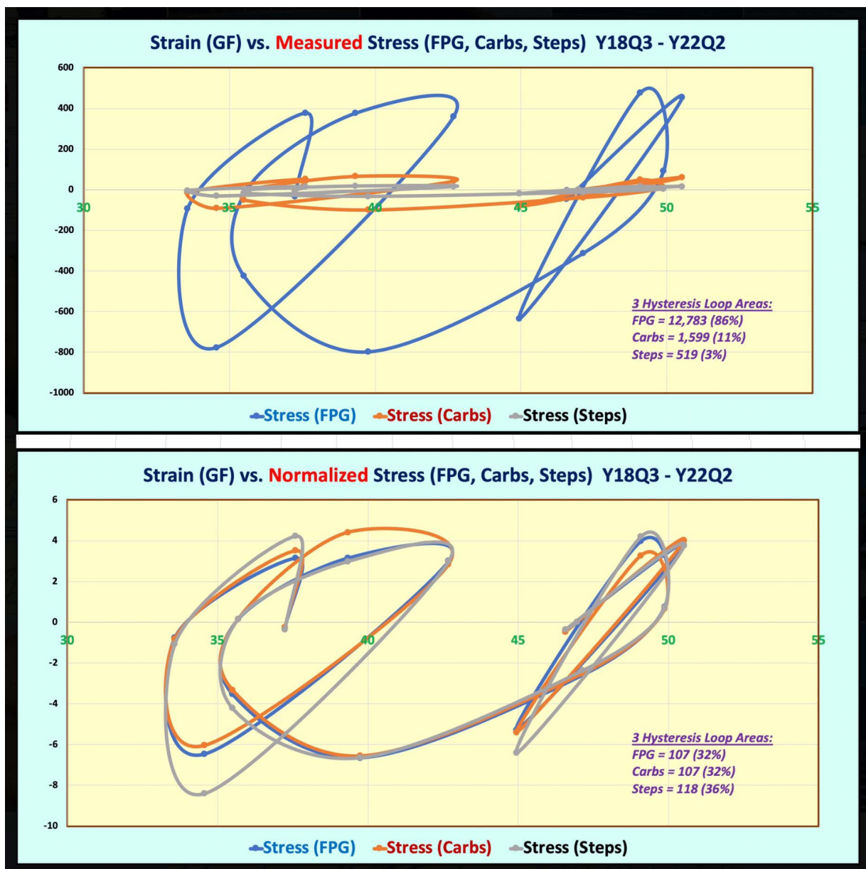
Figure 2: 2 VGT stress-strain diagrams & hysteresis loop areas
