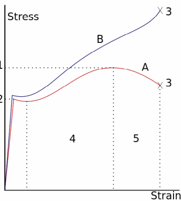
A stress-strain curve typical of structural steel.
