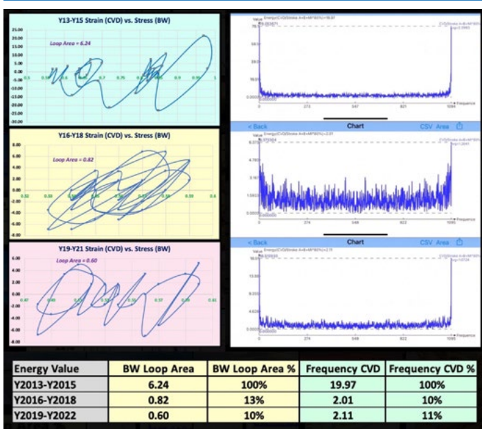
Figure 2: 3 stress-strain diagrams for CVD risk versus BW and three frequency energy diagrams of three triple-year sub-periods with a comparison energy data table
