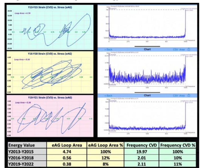
Figure 1: 3 stress-strain diagrams for CVD risk versus eAG and three frequency energy diagrams of three triple-year sub-periods with a comparison energy data table
