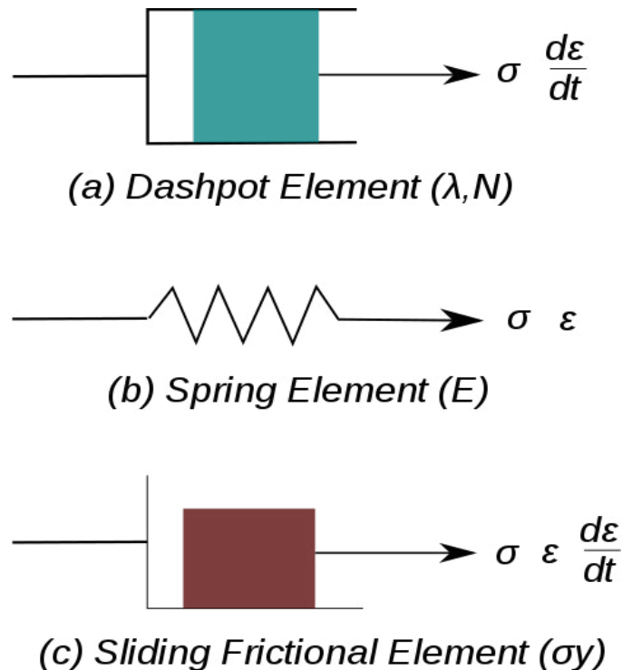
Figure 1: Elements used in one-dimensional models of viscoplastic materials.
