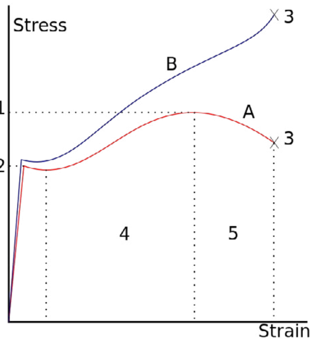
A stress-strain is typical of structural steel.
