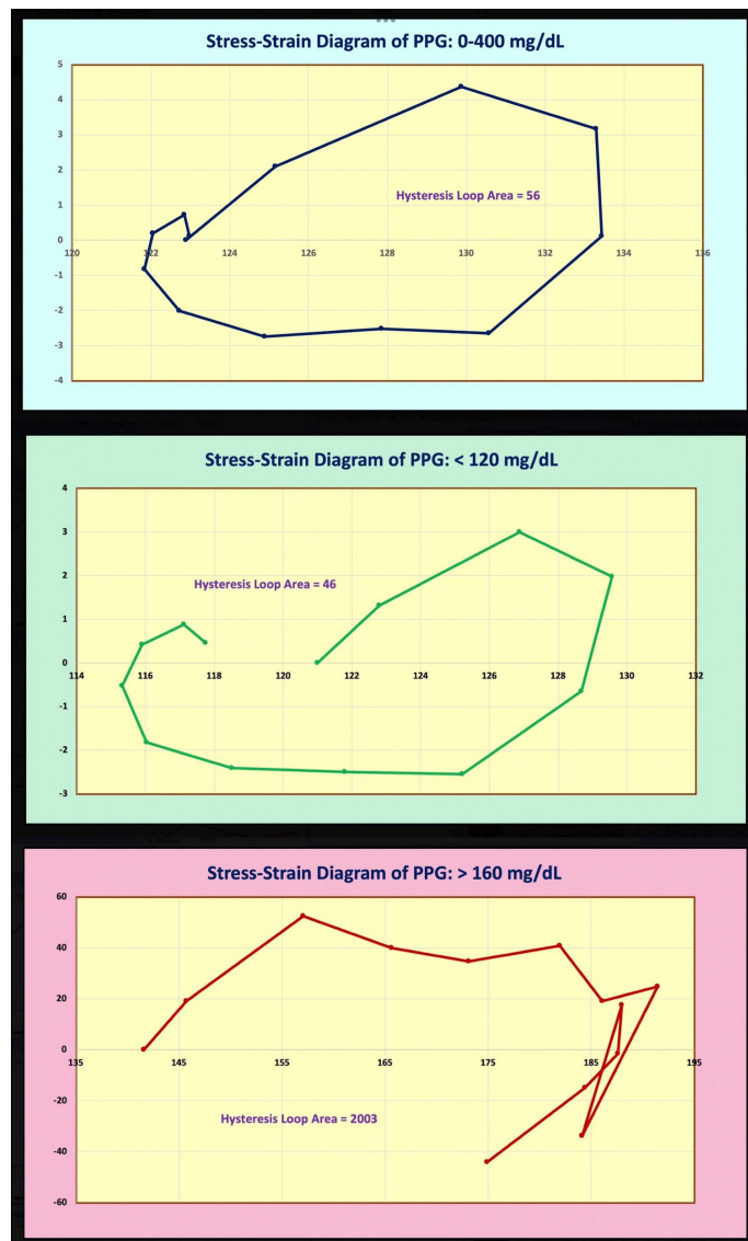
Figure 2: Comparison of stress-strain diagrams of 3 PPG cases
