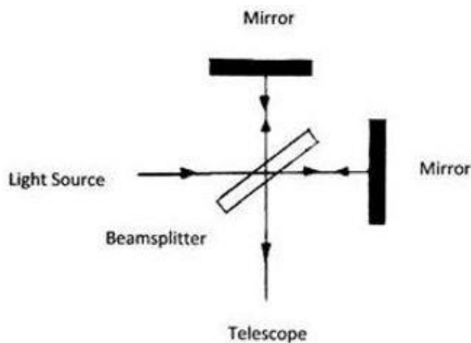
Figure 4: Michelson-Morley apparatus
