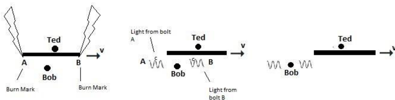
Figure 6: An Experiment to Study Simultaneity. Ted is Moving to the Right with Velocity V.
