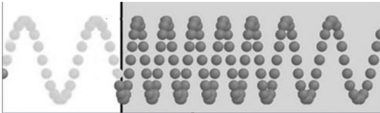
Figure 10: Photons in Red and Blue Light Wave
