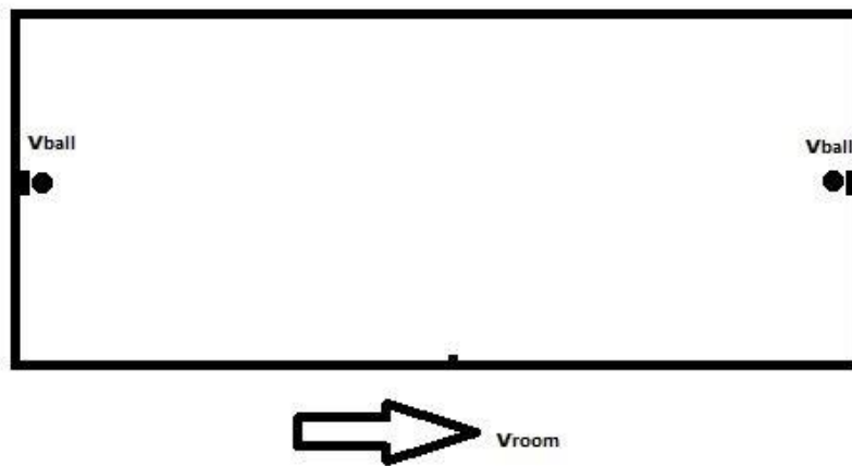
Figure 1: Room Moving to Right with Velocity v
