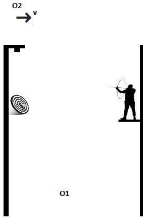
Figure 6 : An Archer is Throwing an Arrow on Target
