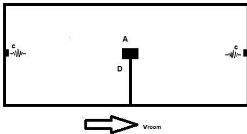
Figure 2: Room Moving with Velocity to the Right and a Detector
