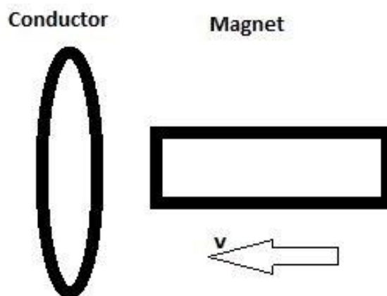
Figure 5: Magnet Moving Towards Conductor
