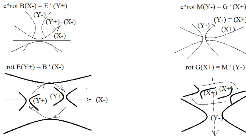
Figure 5: Unified Fields of Space-Matter
