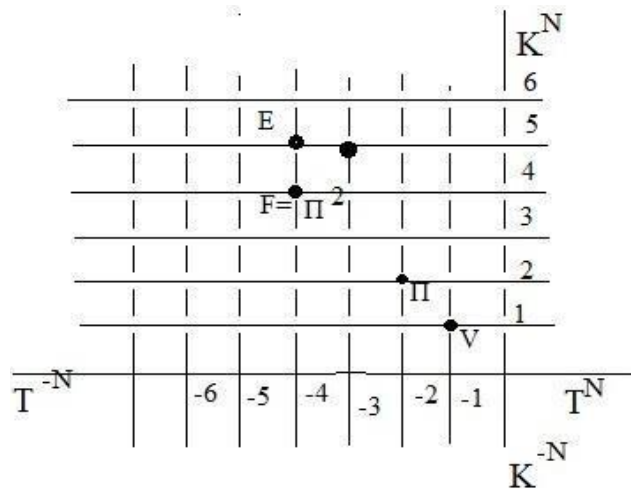
Figure 2: Criteria Of Evolution in Space-Time.
