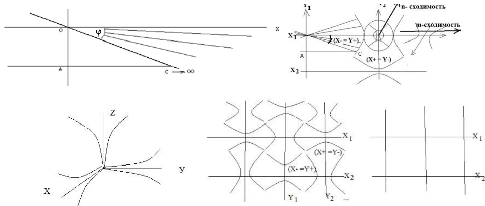
Figure 1: Dynamic Space -Matter.
