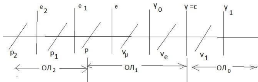
Figure 3: Indivisible Quanta of Space-Matter
