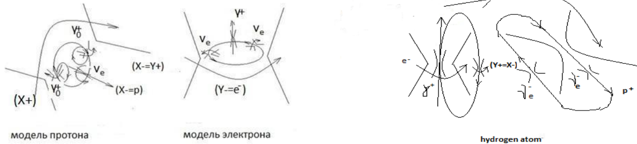
Figure 5: Unified Fields of Space-Matter
