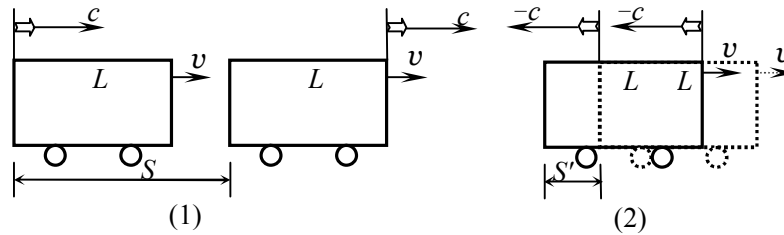
Figure 2: Birds are Flying beside the Car
