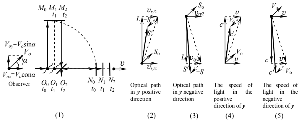
Figure 6: An Observer Observes an Interferometer Moving with the Earth in any Direction in any Reference Frame
