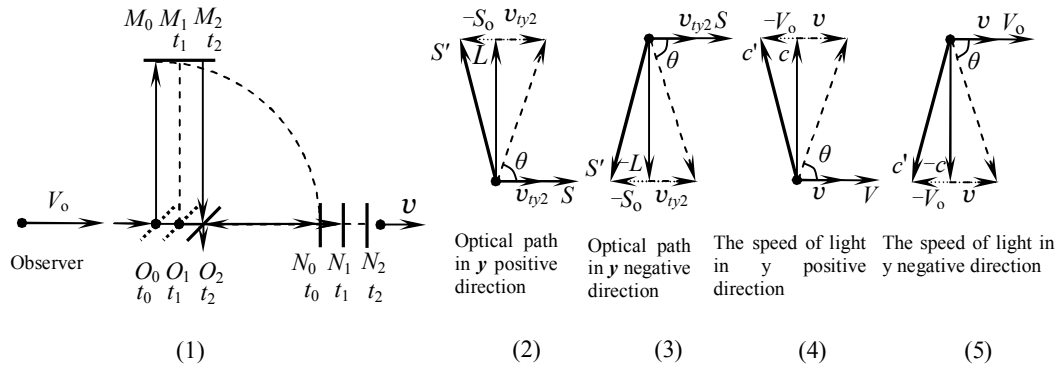
Figure 5: An Observer Observes an Interferometer Moving Along with the Earth in the Positive x Direction in any Reference Frame
