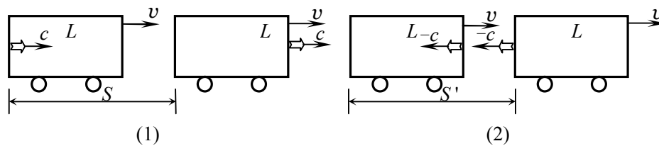
Figure 1: A Bird Flies in the Car
