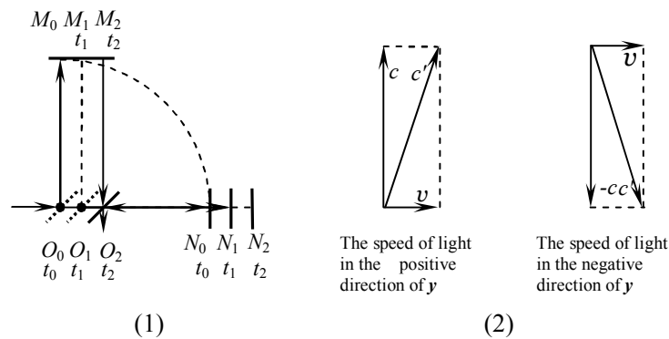
Figure 4: Michelson-Morey Experimental Analysis
