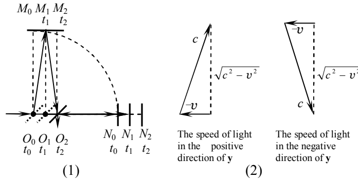
Figure 7: Michelson's Analysis of Michelson-Morey Experiment
