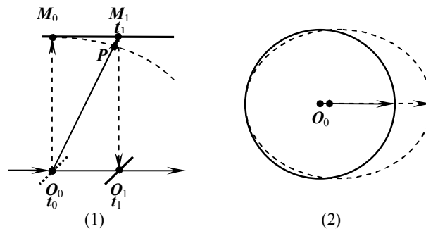
Figure 8: Lorentz Transformation Factor Forcibly Changes the Actual Shape of Light Wave Front
