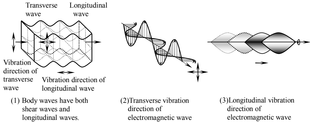
Figure 3: Vibration Direction of Body Wave and Electromagnetic Wave
