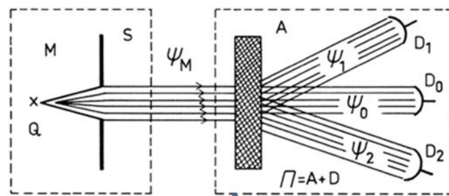
Figure. III.1 Conceptual Scheme of Direct Measurements
