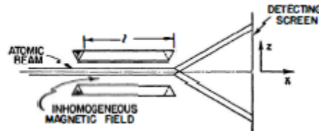
Figure. III.1.1 The Stern-Gerlach Experiment (from Bohm, 1989)
