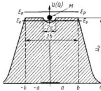
Figure III.2.1 The Energy Profile of Hill With a Ball (from Blokhintsev, 1988)
