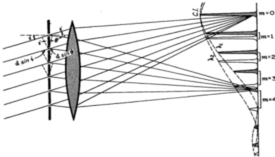
Figure III.1.2 The Classical Diffraction Scheme (from Jenkins, White, 1976)).
