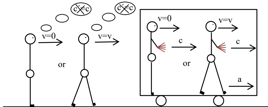
Figure 2: Measurement of the speed of light in different inertial frames (Special Theory of Relativity)
