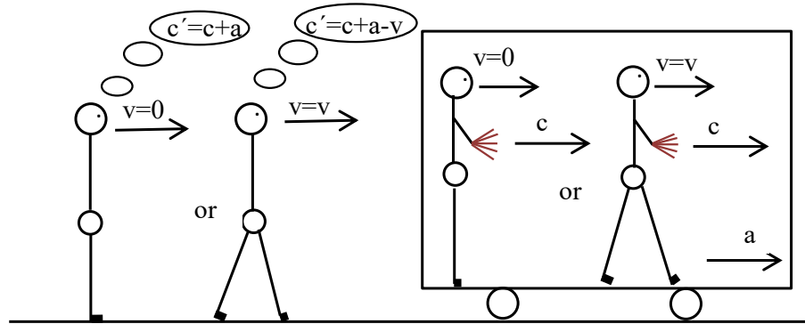
Figure 3: Measuring the Speed of Light in Different Inertial Frames (Classical Mechanics)
