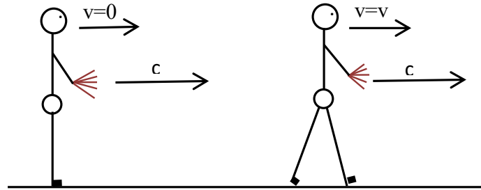
Figure 1: The Constant Speed of Light “ C ” From A Stationary or A Moving Light Source (Special Theory of Relativity and Classical Mechanics)
