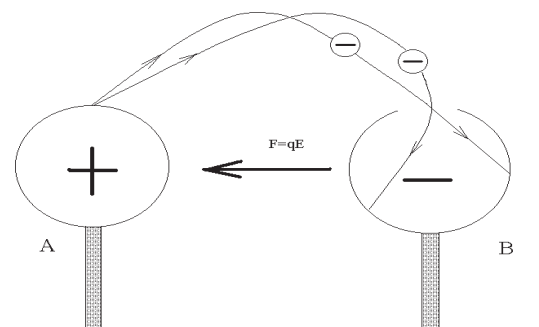
Fig. 8. Work for transferring the charge depends on the mode of transferring and on the path.
