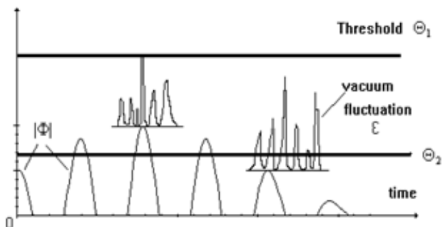
Fig.4. Quantum measurements.
