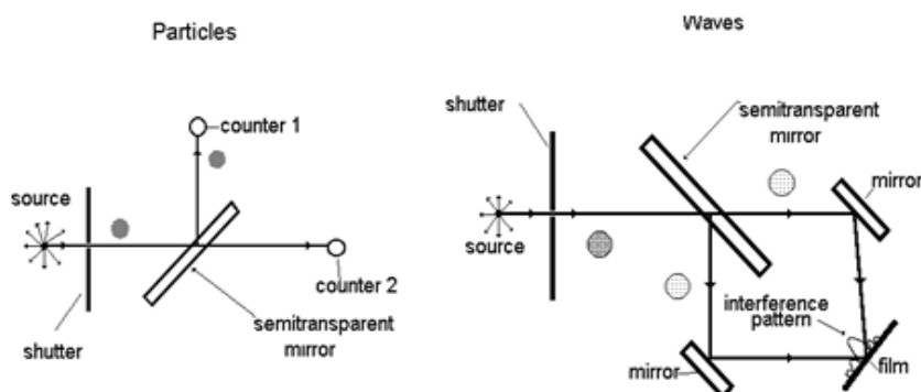
Fig.1. Experiments with individual photons on semitransparent mirror.
