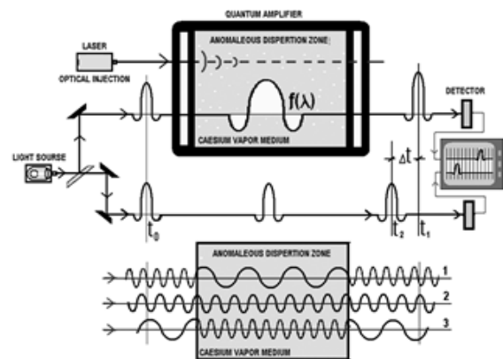
Fig. 5. Experiments of L.Wang - superluminal light propagation.
