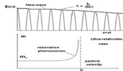
Fig. 3. This is a new wave. And that can be checked experimentally in CERN.
