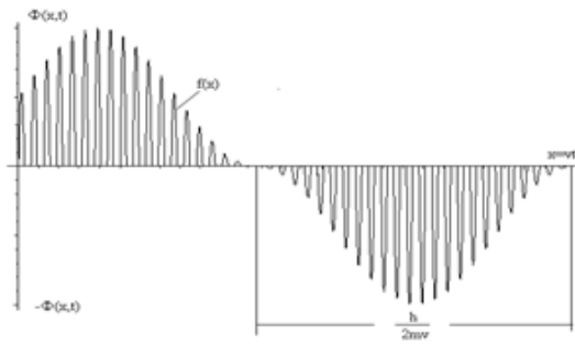
Fig. 2. Behavior of wave packet in linear dispersion medium (i.e., rather like a series of stroboscopic photographs).
