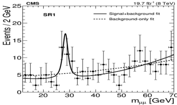
Fig.6. Peak of energy at 28GeV
