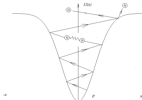
Fig.8. Oscillation of Nitrogen molecule in potential well of catalyst.
