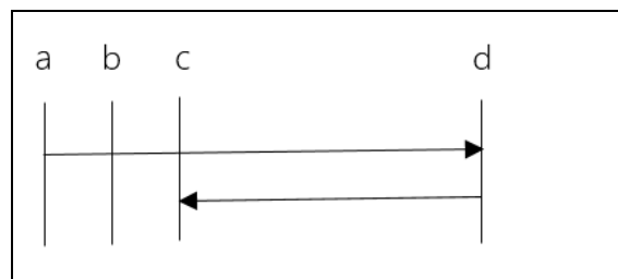
Figure 2: Predict (Or Explain) The Experimental Results of MM Using the Assumption That the Speed of Light Remains Constant in Absolute Space and Lorentz Transformation
