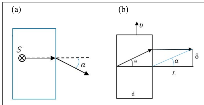
Figure 1 (a): Schematic diagram of the working principle of a speedometer with both an electron gun and a light source embedded in a glass disk (standing on a glass plate and observing). (b): Schematic diagram of Jones experiment. Observe in the laboratory. \theta > \alpha . L is the arm length, and d is the thickness of the glass disk.
