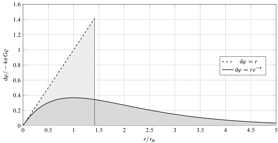
Figure 1: The values which each spherical shell of radius r contributes to the potential of the universe. The total potential \phi(t_u) is equal to the area below the curve. Dashed line: Rigid sphere with finite radius, solid line: universe of the variable speed of light
