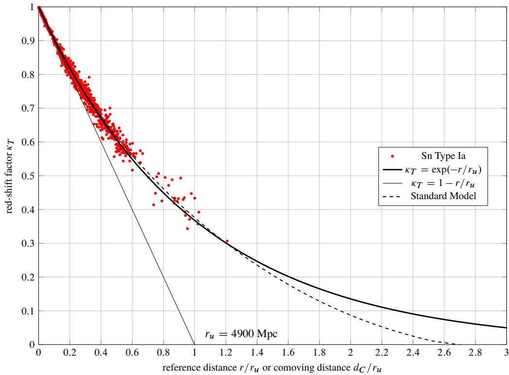
Figure 5: The Hubble diagram represented by the red-shift factor \kappa_T as a function of the reference distance r or the comoving distance d_C , respectively. Near supernovae are tightly compressed in the upper left corner of the graph, the representation of the trend at high red-shifts is very sensitive in return.
