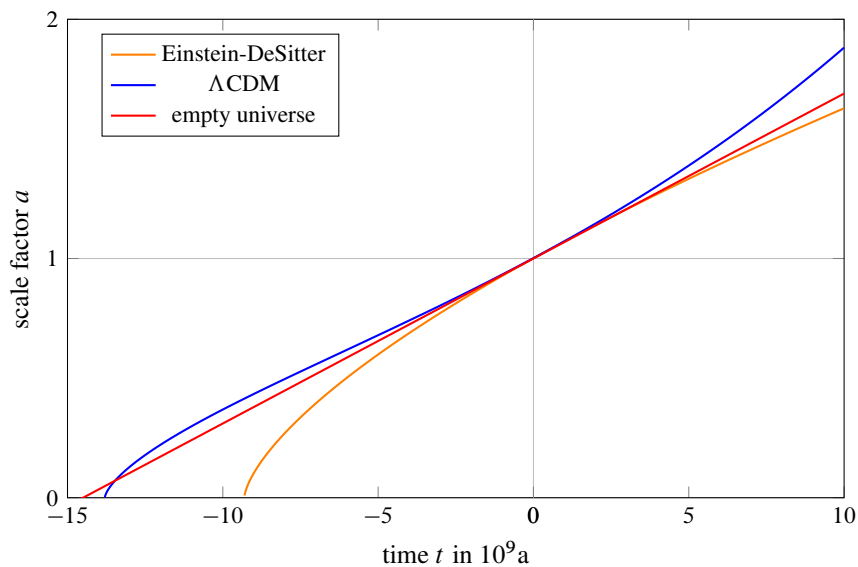
Figure 6: The scale factor of the Standard Model has approximately the same development as the so called “empty universe”, which corresponds to the model of the variable speed of light
