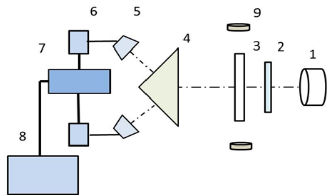
Figure 1: The scheme of measurements of characteristics of the magnetically sensitive layer with magnetic nanoparticles: 1 - semiconductor laser, 2 - polarizer, 3 - liquid-crystal sample, 4 - polarization prism Senarmon, 5 - two photodetectors, 6 - two amplifiers, 7 - two-channel analog-digital converter, 8 - personal computer, 9 - Helmholtz coils
