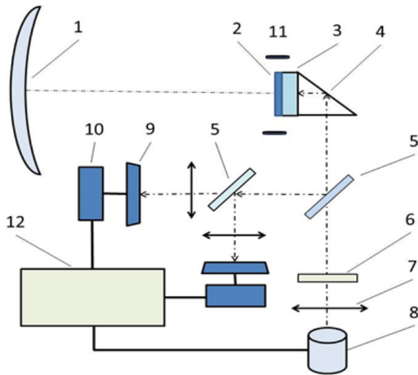
Figure 5: Scheme of the system for detection of inhomogeneous magnetic field. 1 - spherical mirror, 2 - nonmagnetic reflective layer, 3 - magneto-sensitive liquid crystal sensor, 4 - totally reflecting prism, 5 - two interference polarization mirrors, 6 - polarizer, 7 - lens system, 8 - laser, 9 - two photodetectors matrix type, 10 - two blocks of amplification and signal conversion, 11 - magnetic field source, 12 - control and data processing unit.
