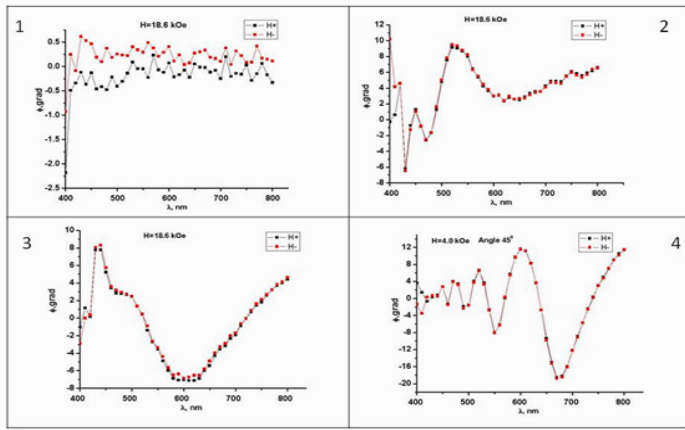
Figure 2: The effective value of the angle of rotation of the plane of polarization of linearly polarized light after passing through the nematic liquid crystal: 1 – nonoriented liquid crystal without magnetic nanoparticles; 2 - nonoriented liquid crystal with magnetic nanoparticles \text{Fe}_2\text{O}_3 ; 3 - oriented liquid crystal without magnetic nanoparticles; 4 - oriented liquid crystal with magnetic nanoparticles \text{Fe}_2\text{O}_3
