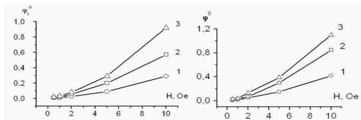
Figure 3: Dependence of the angle of rotation of the director of oriented liquid nematic crystals with magnetic nanoparticles on the intensity of the measuring H_i magnetic field at different concentrations magnetic nanoparticles (I - N=3\% , II - N=5\% ) and at different values of reference magnetig field H_0 : 1- H_0=1 \text{ Oe} , 2- H_0=10 \text{ Oe} , 3- H_0=20 \text{ Oe} .
