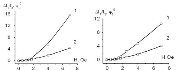
Figure 4: The difference of photoelectric signals \Delta I_1(H)/I_2(0) and the value of the angle \varphi(H) induced by the measuring pulsed magnetic field H_i : 4-I - the value of the angle \varphi(H) was calculated by expression (7.1), 4-II - the value of the angle \varphi(H) was calculated by expression (7.2), the amplitude of magnetic bias field is 2 \text{ Oe} .
