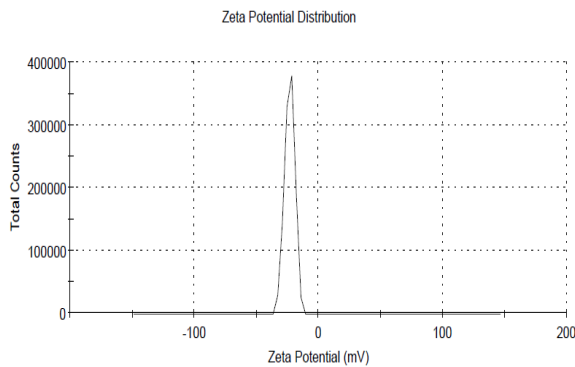
Figure 21: Results for untreated soil (From graph value of Zeta potential is -23.3mV)
