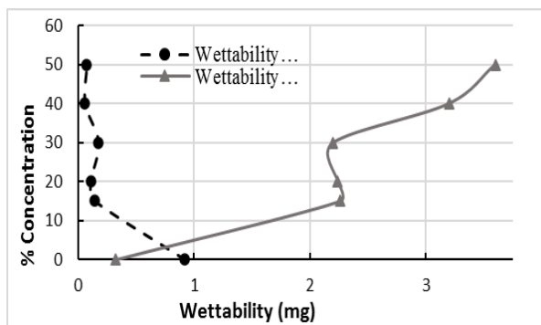
Figure-28: Comparison of wettability of water and oil
