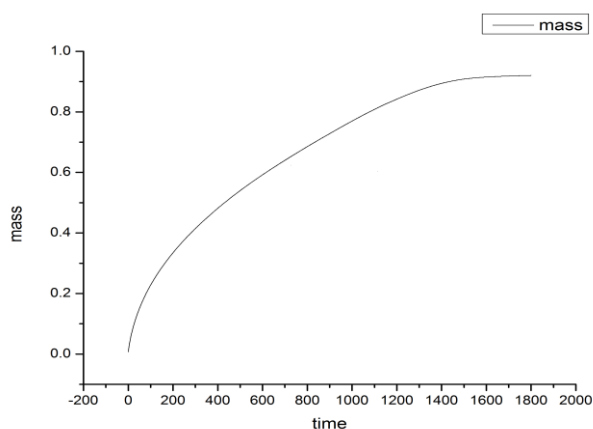
Figure-25: Results for untreated soil (water absorbed is 0.921mg)
