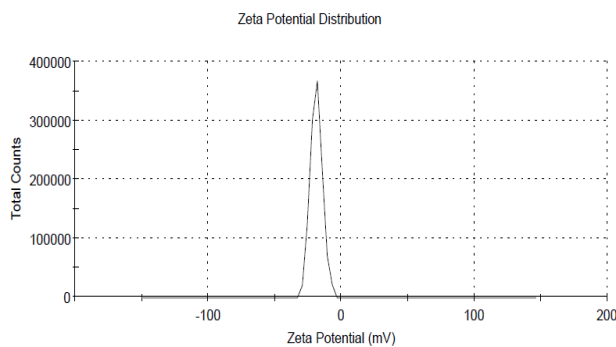
Figure-23: Results for soil treated with 40% concentration ones (From graph value of Zeta potential is -18.8mV)
