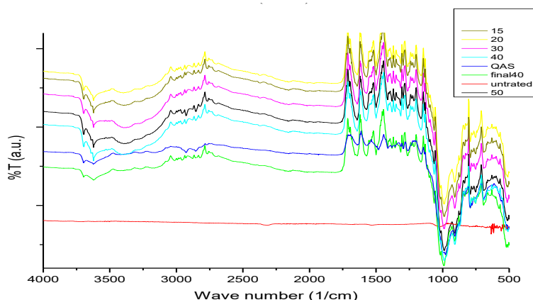
Figure 11: Fourier- transformation infrared (FTIR)
