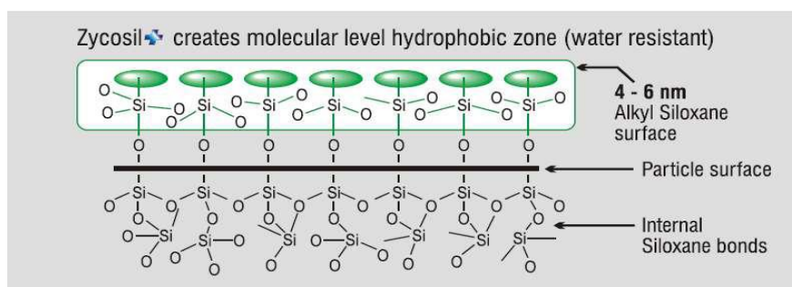
Figure 1: Schematic diagram for Zycosil treated silicates
