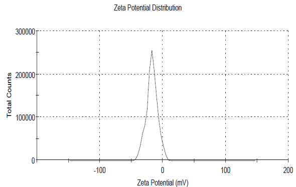
Figure 22: Results for soil treated QAS (From graph value of Zeta potential is -17.3mV)
