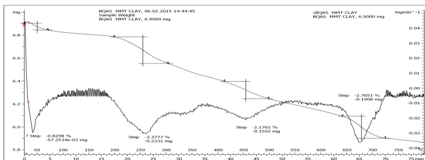
Figure 13: Results for soil treated with QAS
