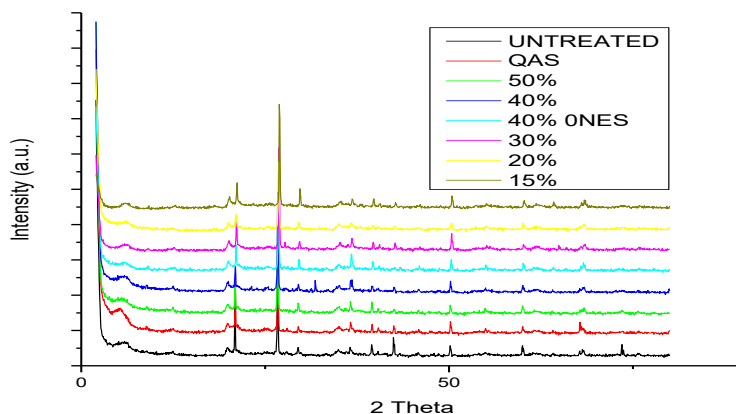
Figure 19: X-ray diffraction spectroscopy
