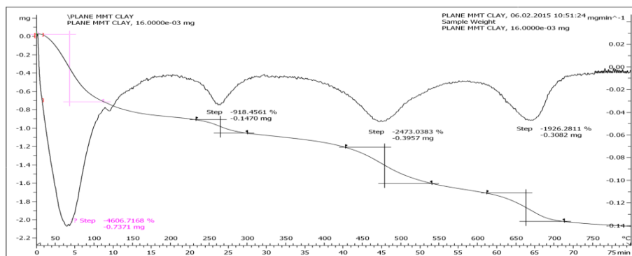
Figure 12: Results for untreated soil
