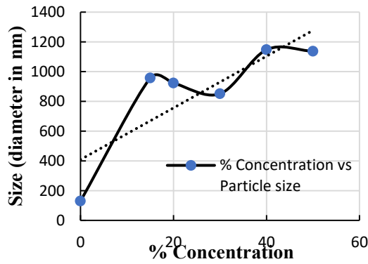
Figure 20 Particle size (diameter in nm) vs % concentration
