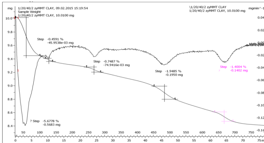
Figure 17: Results for soil treated with 40% concentration twice
