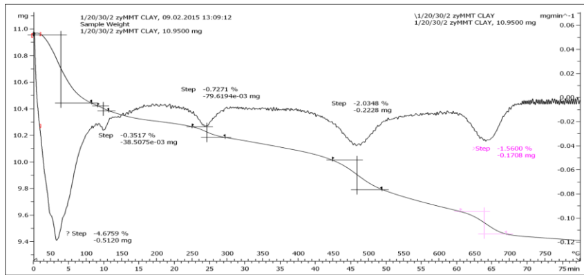
Figure 16: Results for soil treated with 30% concentration twice
