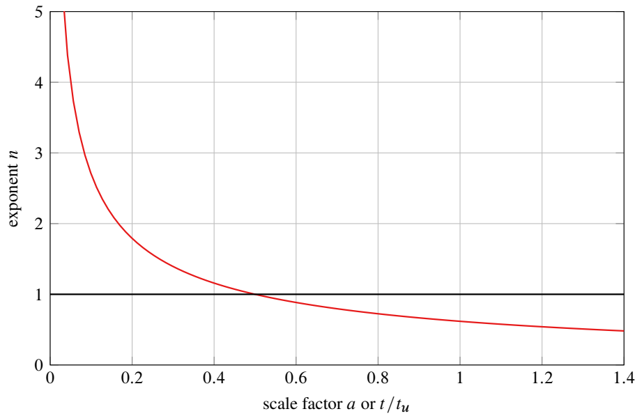
Figure 2: The Evolution of the Exponent N of the Density Fluctuations
