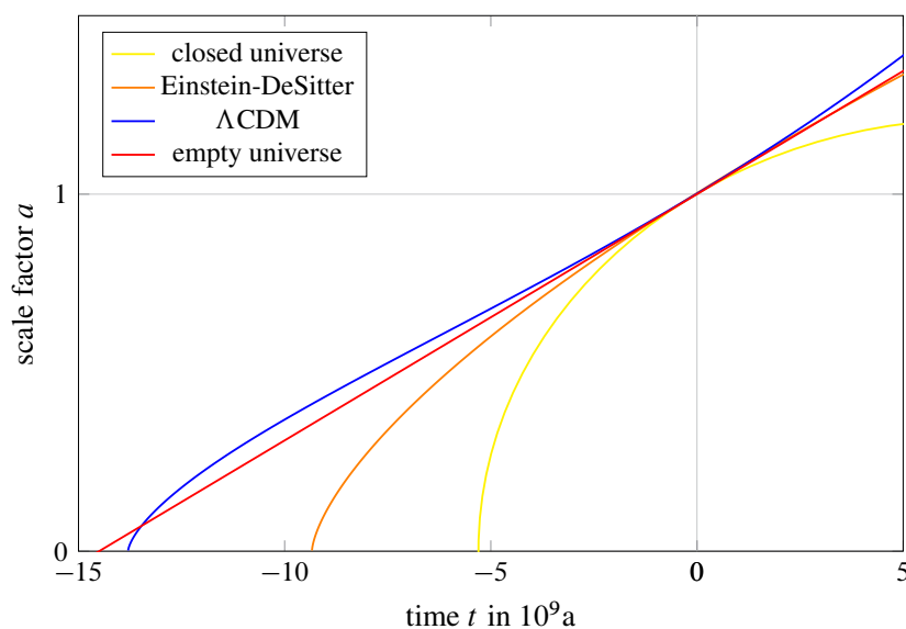
Figure 1: The Development of the Scale Factor According Different Models
