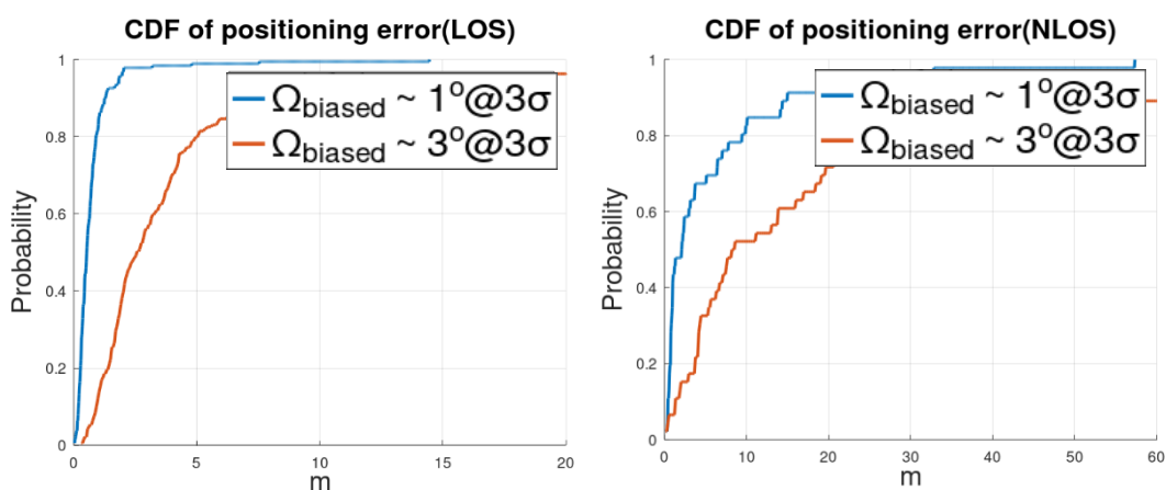
Figure 10: CDF of error of joint estimation of the most likely position
