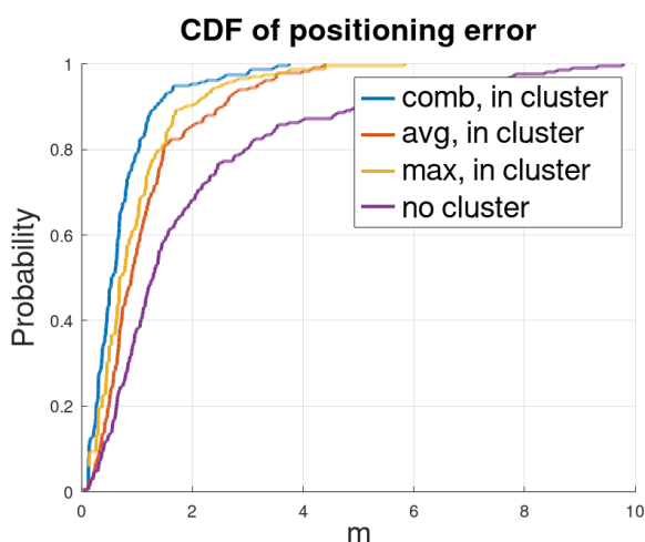
Figure 11: CDF of Error of Joint Estimation of Expected Position with Main Cluster Selection
