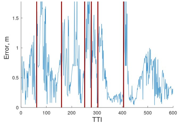
Figure 14: Absolute tracking error across the track (Figure 13). Vertical lines correspond to the moments when UE turns in another direction
