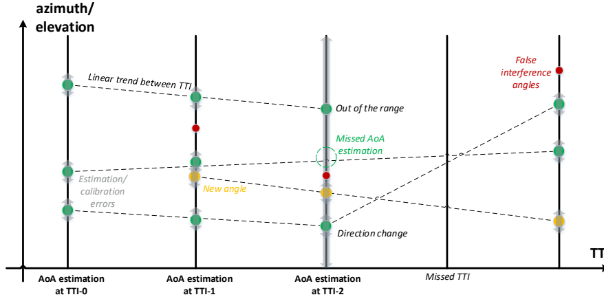
Figure 6: Assumptions for Angle Tracking Model
