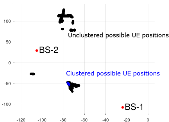
Figure 12: Example of clustering of candidates for UE position
