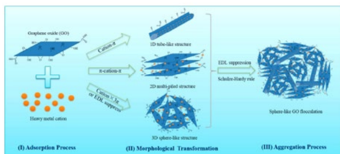
Figure 11: from Environ. Sci. Technol. 2016, 50, 20, 11066-11075 Proposed interactions of heavy metal cations with GO nano sheets in 3 steps: (1) adsorption of heavy metal onto GO nano-sheets; (2) formation of 1D-, 2D-, and 3D-like structures; and (3) aggregation of sphere-like flocculation.
