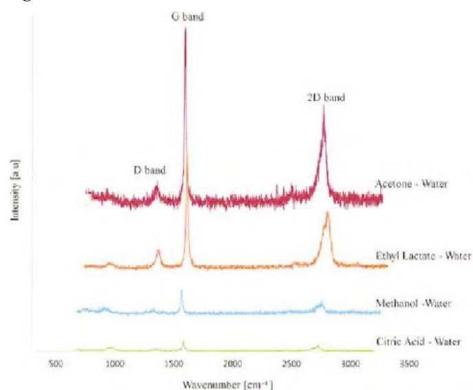
Figure 10: Raman spectra RS of graphene exfoliated via different solvent systems. An increase in the D peak is observed as
