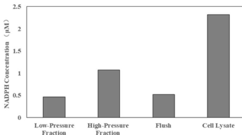
Figure 3: NADPH concentration in the low-pressure fraction (< 0.8 bar), the high-pressure fraction (> 0.8 bar), the flush of the depth filtration, and the cell lysate of the molecule 2 cell culture
