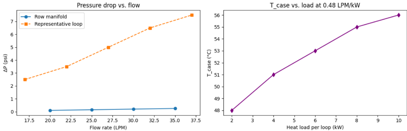
Figure 3: (Left) Measured Pressure Drops vs. Flow for Row Manifold and Representative Rack Loop (Right) Heater case temperature vs. load at fixed flow (0.48 LPM/kW). Note: Where raw arrays were unavailable, synthetic points were constructed to match reported extrema and trends.
