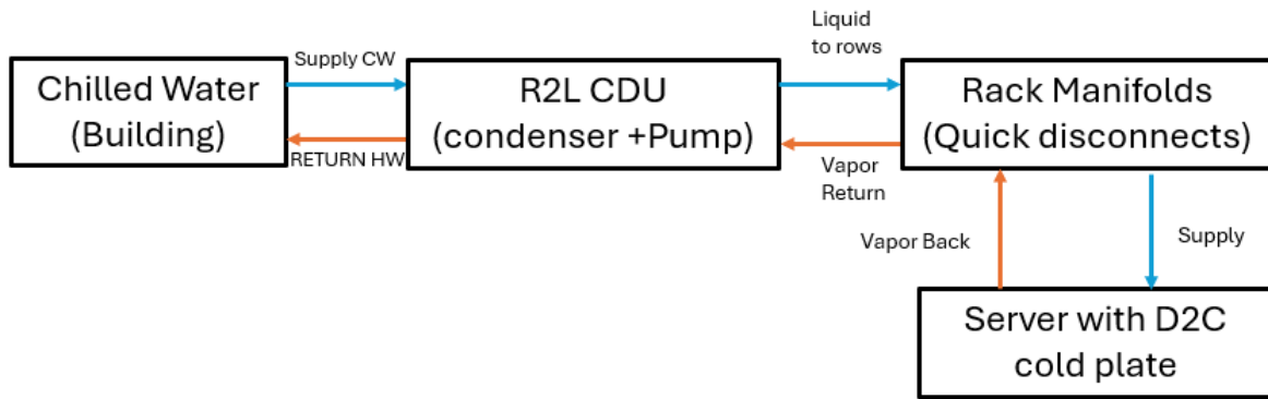
Figure 1: Conceptual R2L Pumped Two-Phase Cooling Architecture (Schematic)
