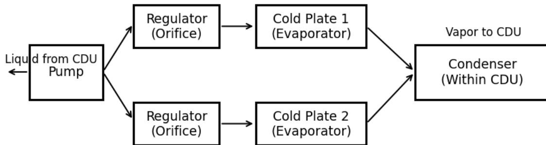
Figure 2: Example Pumped Two-Phase Loop Schematic Showing Parallel Cold-Plate Evaporators and Flow Regulators
