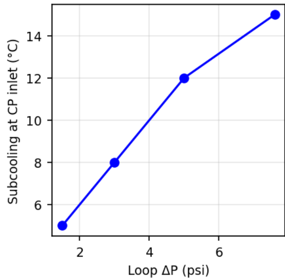
Figure 4: Subcooling vs. loop pressure drop across load
