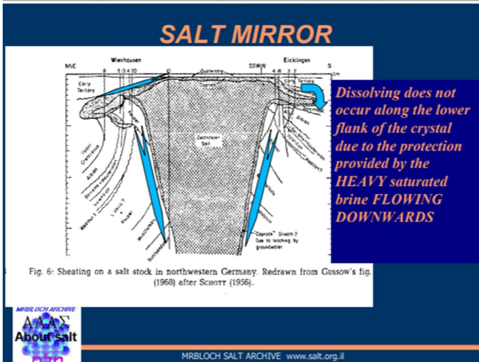
Figure 7: Salt Mirror streams of dissolved salt dragging debris of decomposed organic matter
