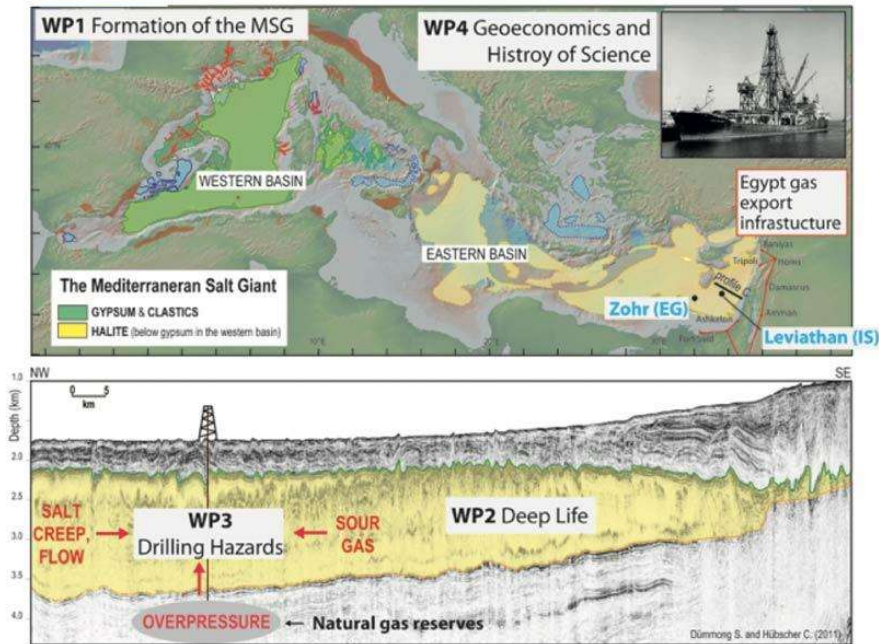
Figure 3: example Salt mirror “Salt Giant” Eastern Mediterranean basin
