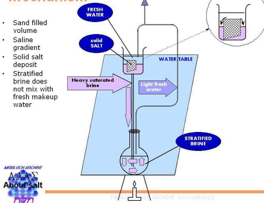
Figure 2: Laboratory cycling of brine in a simulated geothermal saline pool
