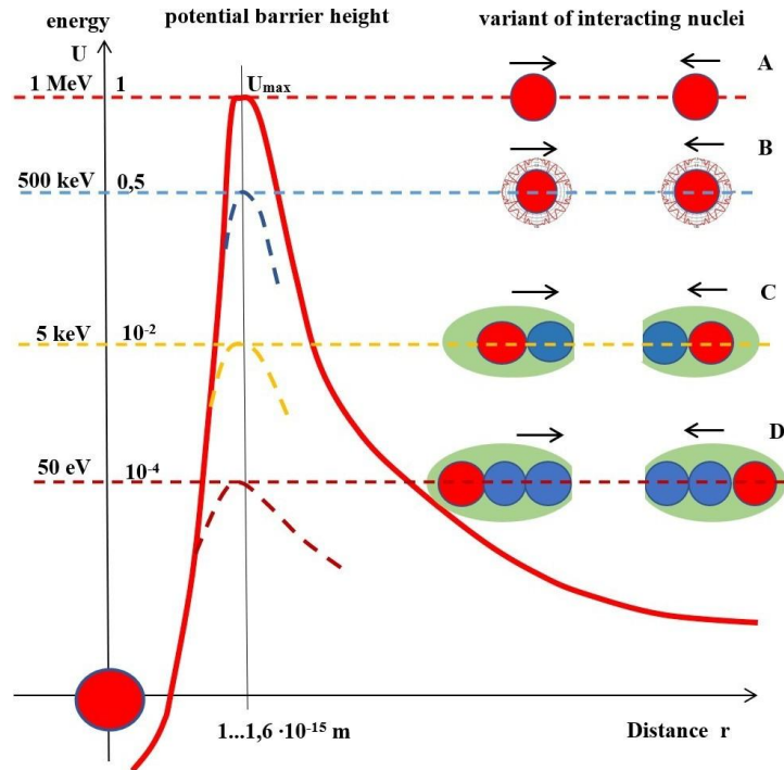
Figure 22: The height of the potential barrier U_{max} of interacting nuclei depends on their structures and spatial orientation at the moment of approach
