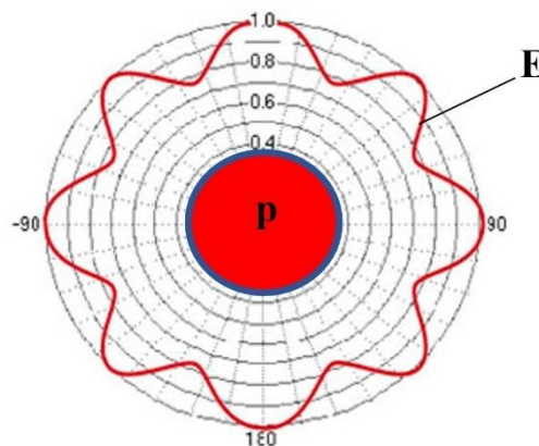
Figure 8: Cross section of the proton's electric field E at a distance of the Coulomb barrier (changes in the surface charge density of the proton lead to oscillation of its electric field).
