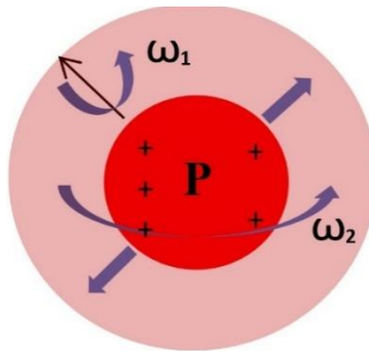
Figure 9: Oscillatory and rotational motions of the proton in the nucleus lead to additional fluctuations of the electric field E of the proton.
