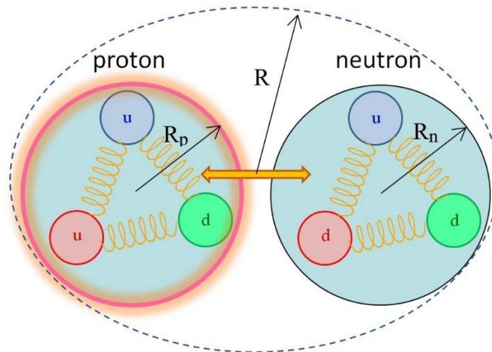
Figure 6: Structure of nucleons (simplified version): proton consists of two top quarks U with charge +2/3 e and one bottom quark d with charge -1/3 e , neutron consists of two lower quarks d and one upper quark U , the radius of the proton and neutron R_{pn} \sim 4.5616 \cdot 10^{-16} m .
