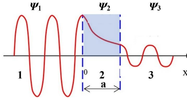
Figure 3: View of \Psi -functions (de Broglie waves) for different regions when microparticles pass through the potential barrier ( \psi_1 - de Broglie wave with frequency f and amplitude A_1 , \psi_2 \neq 0 , \psi_3 - de Broglie wave with frequency f and amplitude A_3 < A_1 ).
