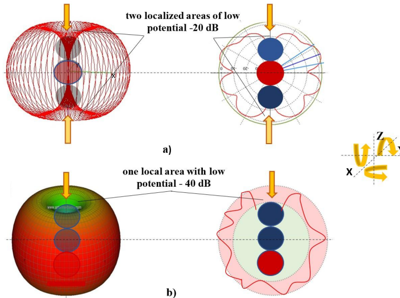
Figure 20: Low-potential channels are formed in the Coulomb field of the tritium nucleus and provide probable passage of microparticles into the nucleus:
