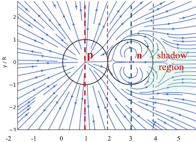
Figure 12: Deuterium Nucleus Model for Estimating the Electric Field and Potential
