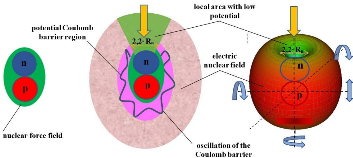
Figure 18: The electric field of the deuterium nucleus oscillates and forms one local low potential region that rotates with the nucleus around the x, y, z axes
