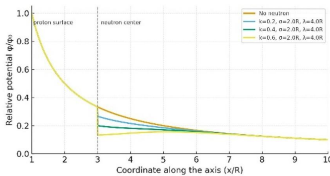
Figure 13: Comparative graphs showing the attenuation of the \varphi/\varphi_0 potential behind the neutron in the near zone: base curves: \varphi_0 \propto 1/x scaled to a value of 1 at \frac{x}{R} = 1 ; vertical lines at contact points x/R = 1 and neutron center x/R = 3 .
