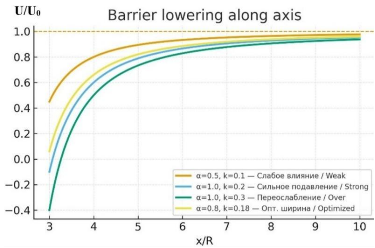
Figure 15: Decrease in the electric field potential of the nucleus U/U_0 under different neutron influence factors: U/U_0 = 1 means that the field is the same as that of a single proton
