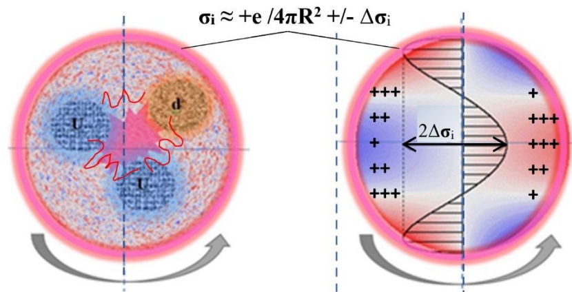
Figure 7: Interactions of quarks U and d in the proton structure lead to a periodic change in the charge density \Delta\sigma_i on the proton surface and a change in the external electric field strength \Delta E , respectively.
