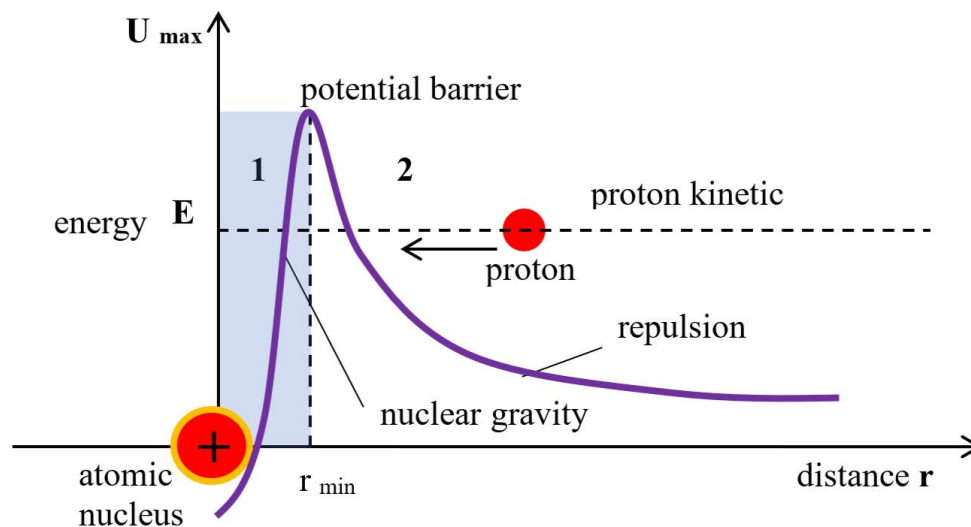
Figure 1: Approximate dependence of the total interaction potential of nuclei on distance has a maximum (the top of the Coulomb barrier) at some distance, and the two regions of space 1 and 2 are separated by a potential barrier
