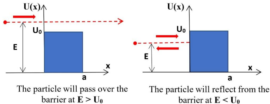
Figure 2: Potential Barrier in the Framework of Classical Mechanics
