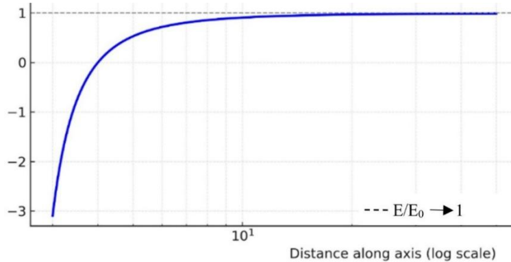
Figure 16: The field strength of the “proton + neutron” system returns to Coulombic
