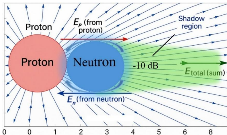
Figure 17: General diagram of the formation of a low-potential channel in the Coulomb field of the nucleus (shadow region) due to the influence of a neutron: red circle - proton (field source); blue circle - neutron (polarizable, uncharged); arrow lines show the direction of the resulting field; on the right, you can see the “shadow zone”, where the field is weakened and partially reversed.
