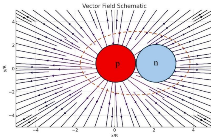
Figure 4 : The electric field of the nucleus without considering the influence of the neutron is a point charge field: the center of the proton is located at axis 0, the center of the neutron is located on axis 2.0, the boundary of the nucleus is at a distance x/R \approx 3.5...4 .
