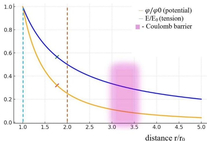
Figure 5: Graph showing the dependence of the field strength and potential of a deuterium nucleus, without considering the influence of the neutron, on the distance along the axis connecting the centers of the proton and neutron: blue line - potential (decreases slowly), orange line - field strength decreases faster).
