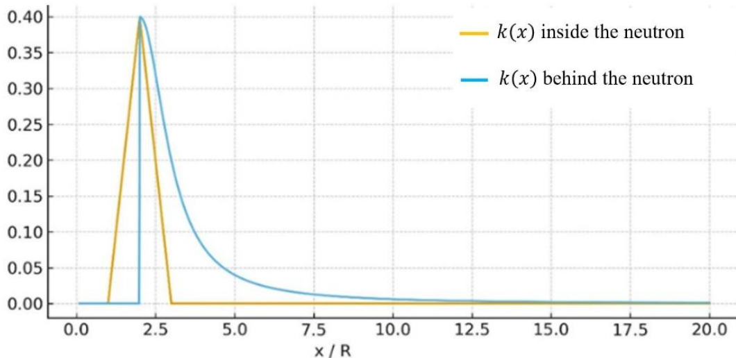
Figure 11: Field Attenuation Profiles Inside the Neutron and Along the Axis Behind the Neutron
