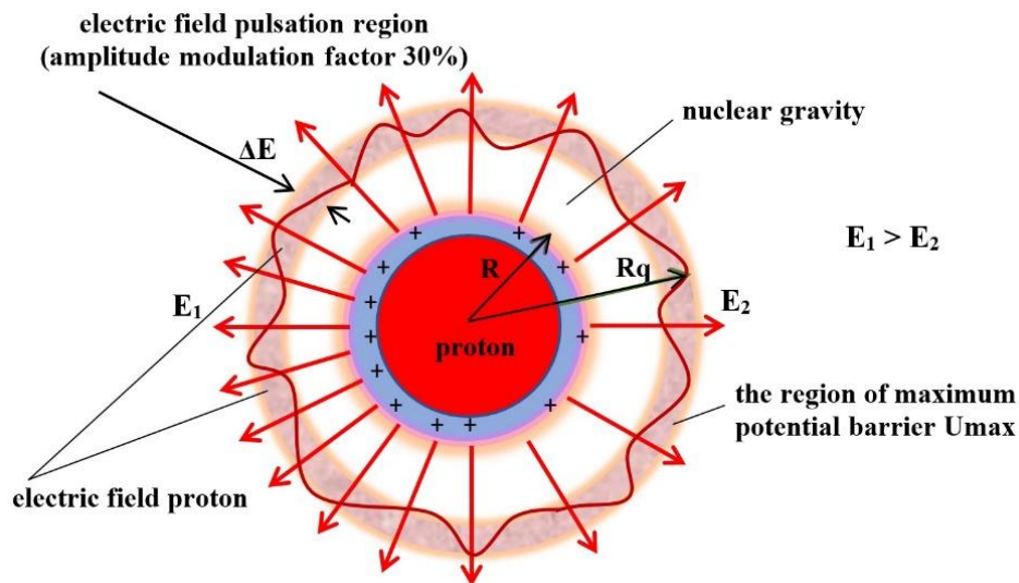
Figure 10: The electric field E of the proton pulsates due to changes in surface charge, mass densities and proton motion
