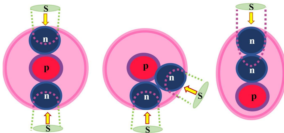
Figure 19: The structure of a tritium nucleus formed from a proton and two neutrons leads to the formation of spatial regions with low potential in the electric field of the proton:
