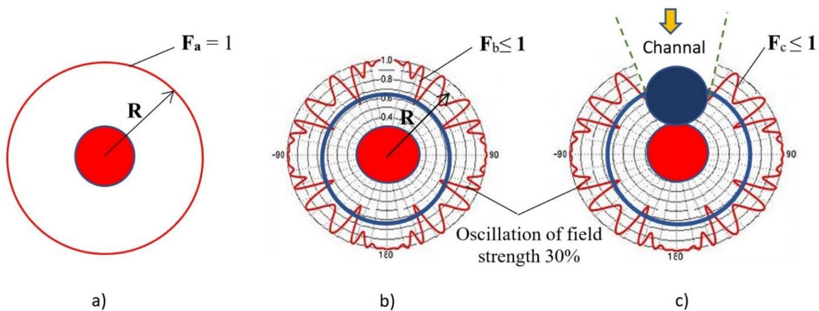
Figure 21: Cross section of normalized ADD F_a , F_b , and F_c electric fields of different nuclei at equidistant distance R from the centers of the nuclei:
