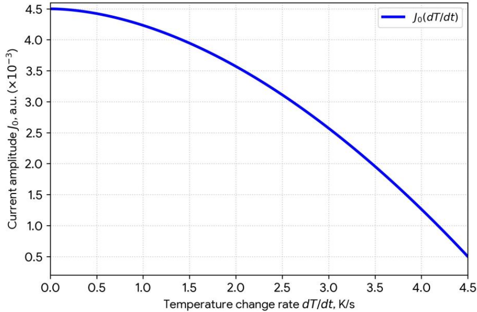
Figure 3: Dependence of the Baseline Amplitude of the Radiation Current on the Macroscopic Heating Rate
