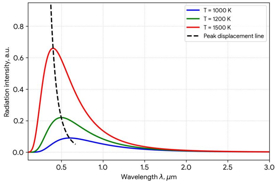
Figure 2: Family of Spectral Curves of Radiation Density of the Medium at Various Temperatures figure[htbp] Dependence of the baseline amplitude of the radiation current on the macroscopic heating rate
