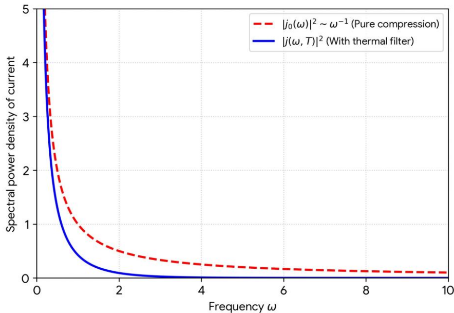
Figure 1: Spectral Power Density of The Electron Cutoff Current as A Function of Frequency
