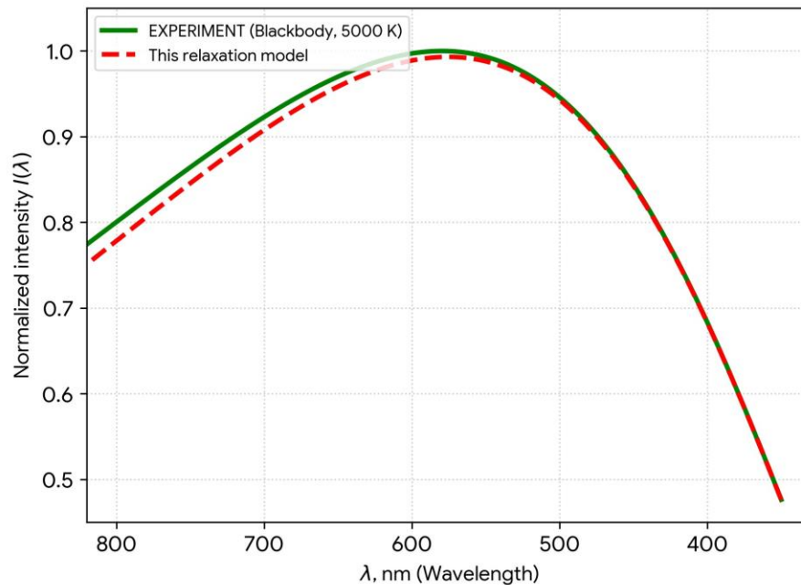
Figure 4: Final Comparison of The Normalized Intensity of The Relaxation Radiation Model with Blackbody Spectral Data ( T = 5000 K)
