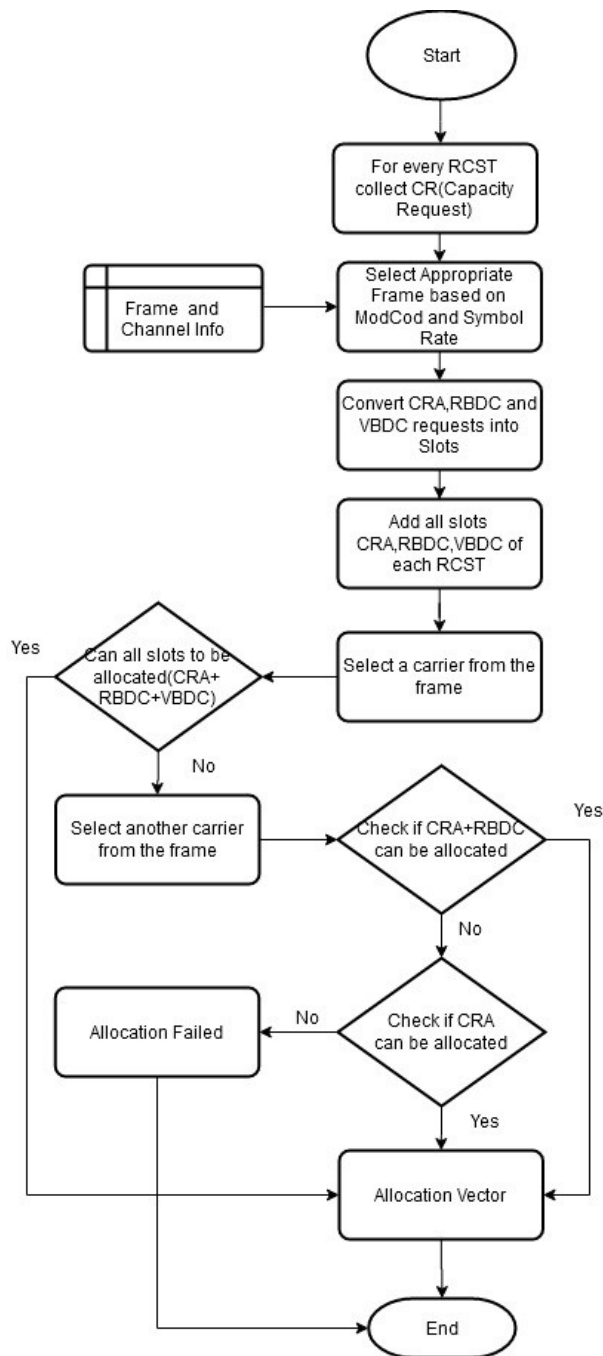
Figure 6: Flow Chart of Resource Allocation Algorithm
