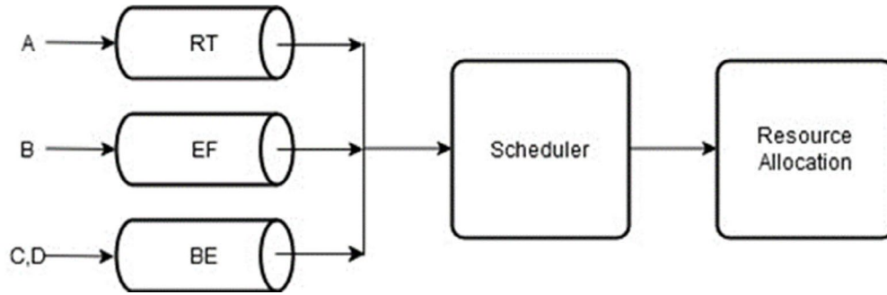
Figure 5: Block Diagram of Priority Queue Scheduling
