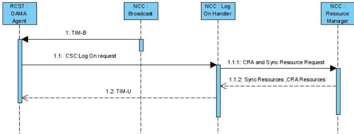
Figure 4: Sequence Diagram of Log on Procedure
