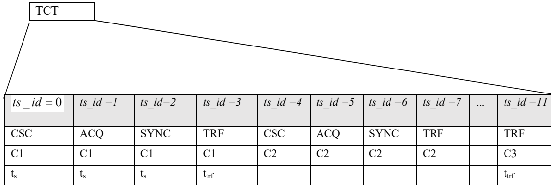
Figure 3: Composition of TCT
