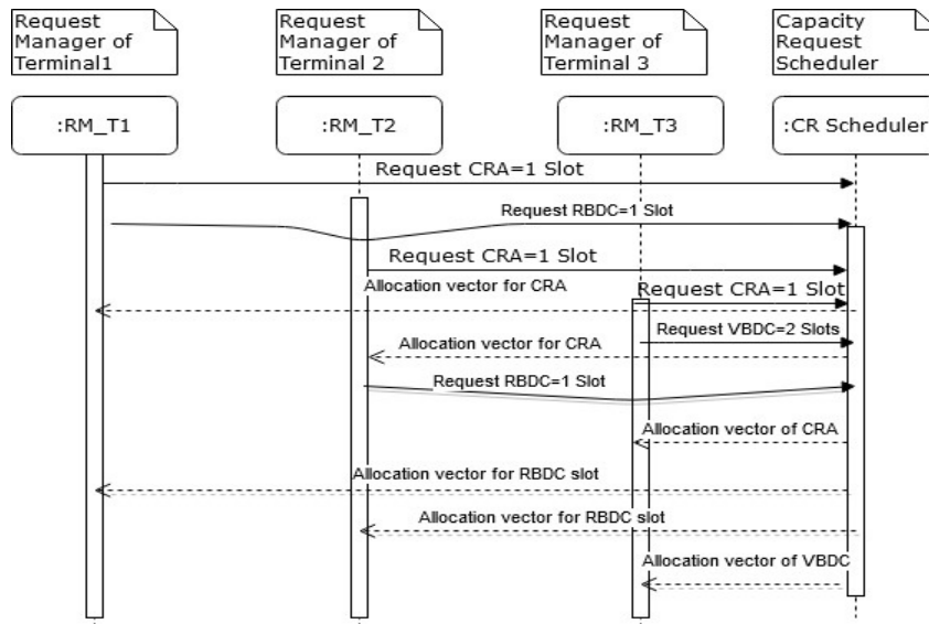
Figure 9: Sequence Diagram of Testing with Three Terminals
