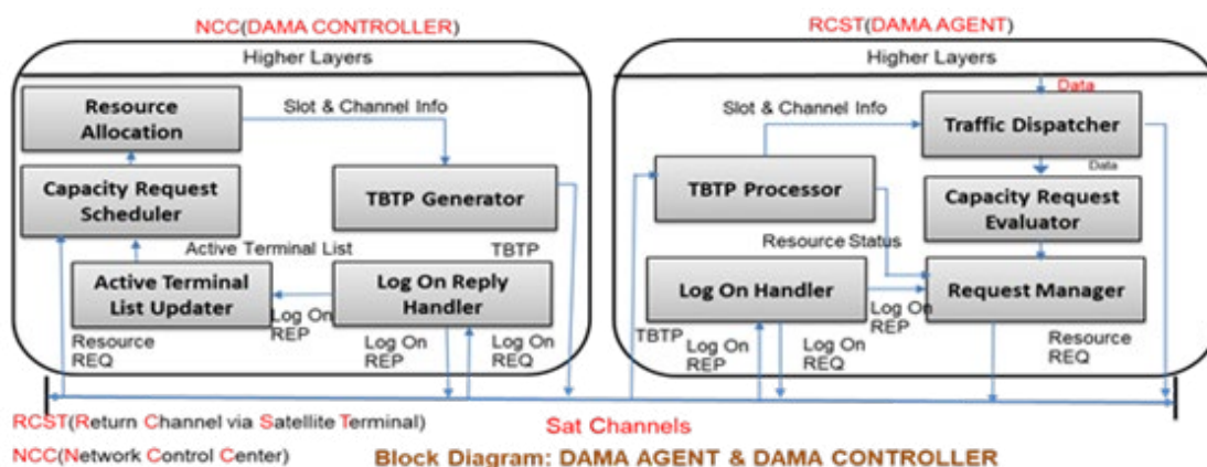
Figure 2: Architecture for Realization of Resource Allocation Method
