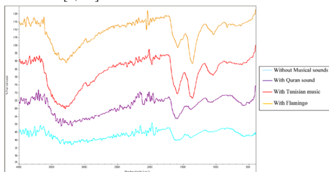
Figure 6: FT-IR Spectrums of Different ZnO NPs Synthesized Using Supernatant of Yarrowia lipolytica .
