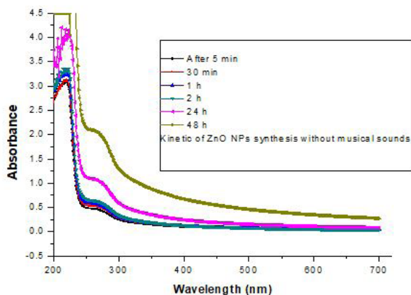
Figure 4: Kinetic of UV/Vis Spectrums of ZnO NPs Synthesized Using Supernatant of Yarrowia lipolytica under Optimum Condition Without Musical Sounds.
