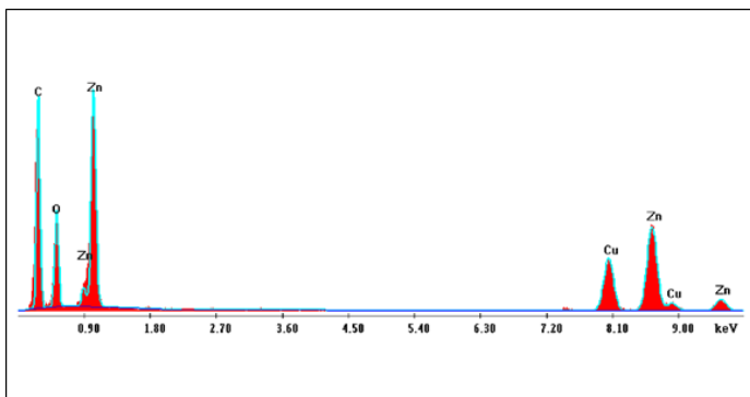
Figure 9: EDX Spectrum of Synthesized Zinc Oxide Nanoparticles.
