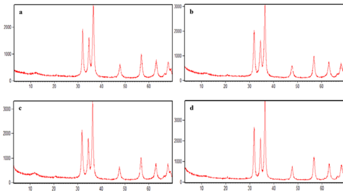
Figure 7: XRD graphs of biosynthesized ZnO NPs using supernatant of Yarrowia lipolytica (a) without musical sounds and with musical sounds (b) Quran sound, (c) Tunisian music, and (d) Flamingo.
