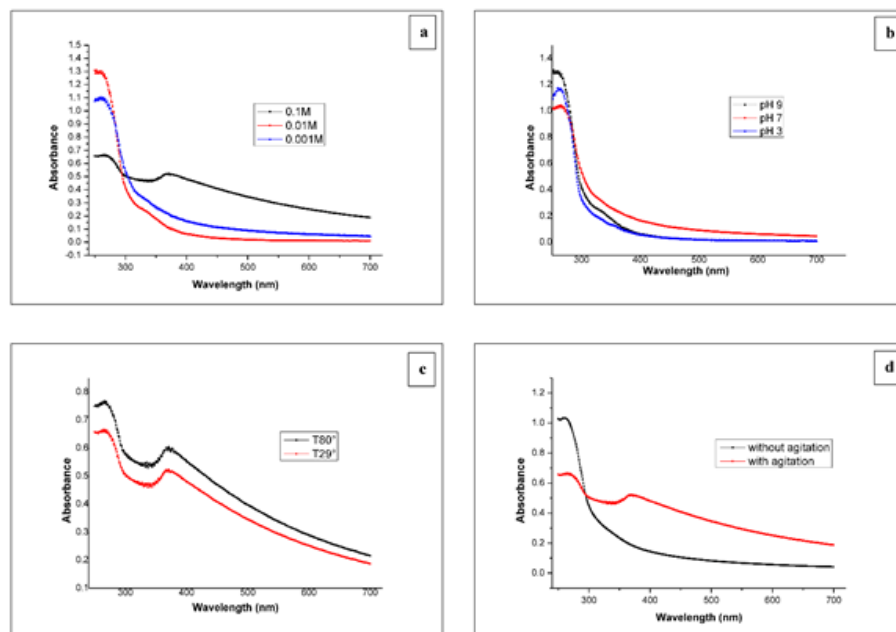
Figure 3: UV/Vis spectrums of ZnO NPs synthesized using supernatant of Yarrowia lipolytica under various (a) concentrations of zinc nitrate, (b) pH, (c) temperature, and (d) static and agitated conditions.
