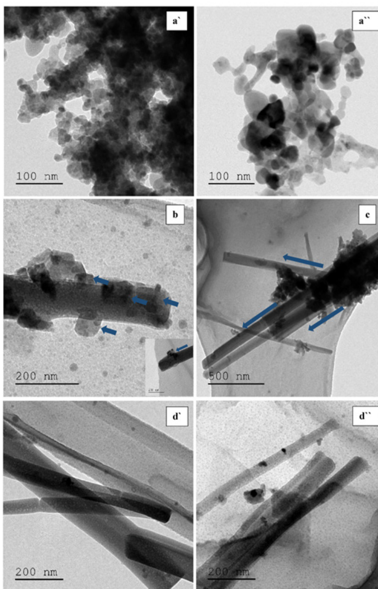
Figure 8: TEM images of the biosynthesized zinc oxide nanoparticles (A', A'') without musical sounds and with musical sounds (B) Flamingo, (C) Tunisian music, and (D', D'') Quran sound.
