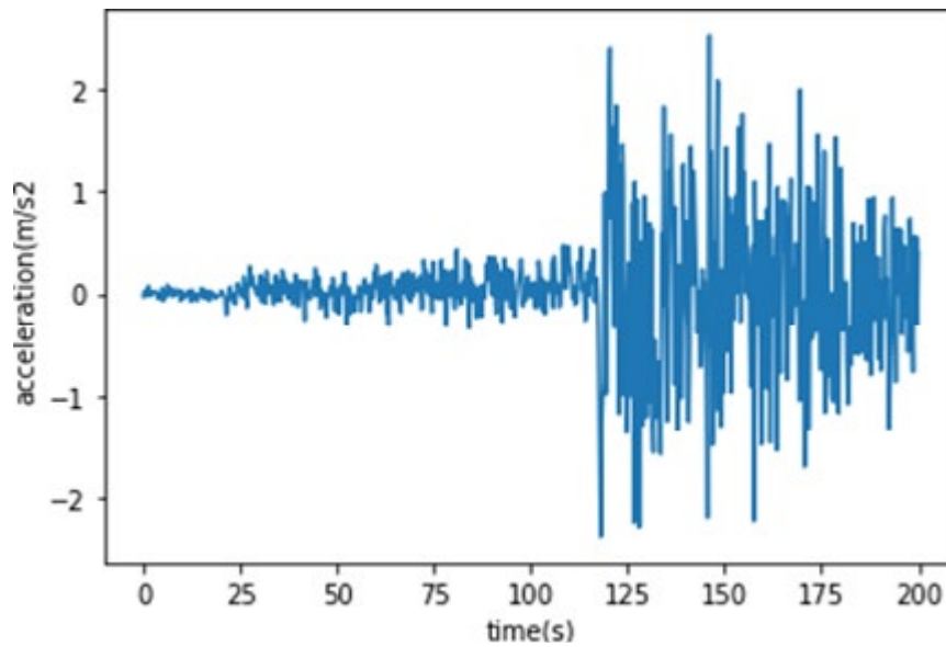
Figure 7: Example of Artificial Seismic Accelerogram For A Sample Of 750 Points, 200s As A Time Interval with Following Statistical Characteristics: Wave Average Standard Deviation P 0.00 0.1 S 0.08 0.154 Surface 0.01 1.20 Envelop 100 100
