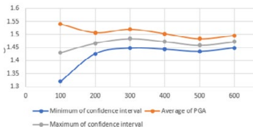
Figure 14: Variation of Average of PGA and Interval of Confidence with Number of Samples
