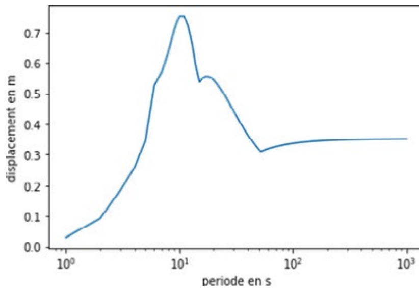
Figure 4: Displacement Spectrum, with D=0.05 , Using Implicit Scheme of Temporal Integration, \beta=1/6 and \gamma=1/2
