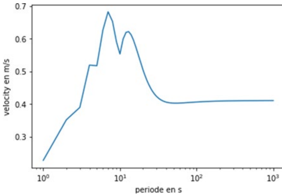
Figure 5: Velocity Spectrum, with D=0.05 , Using Implicit Scheme of Temporal Integration, \text{Beta}=1/6 and \text{Gamma}=1/2
