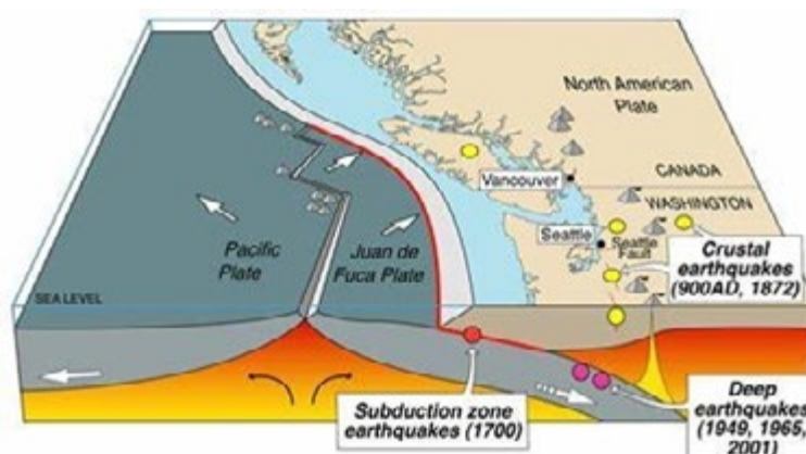
Figure 1: Example of Subduction Zone on Pacific Plate
