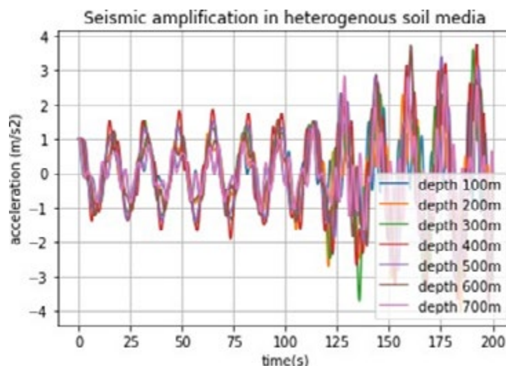
Figure 9: Propagation of Generated Wave Until the Depth of 700m
