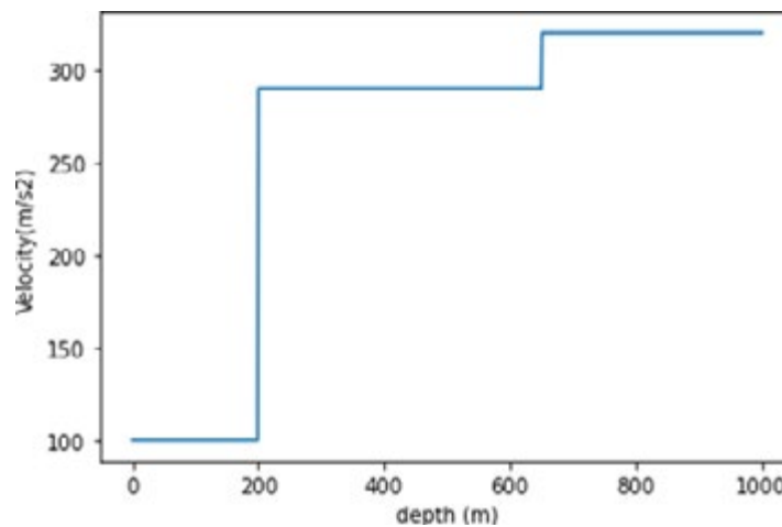
Figure 8: Velocity Diagram to Depth of 1000m:
