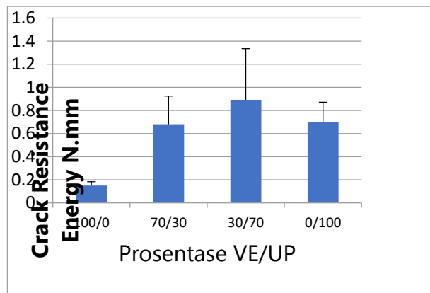
Figure 5: Crack Resistance Energy of UP/VE blends
