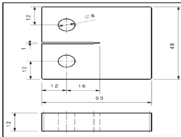
Figure 1: Dimensions of the specimen configuration as used for determining fracture toughness
