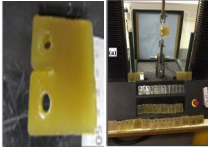
Figure 2: Universal testing machine Autograph Machine Merk COM-TEN 95T Series 5K to crack testing
