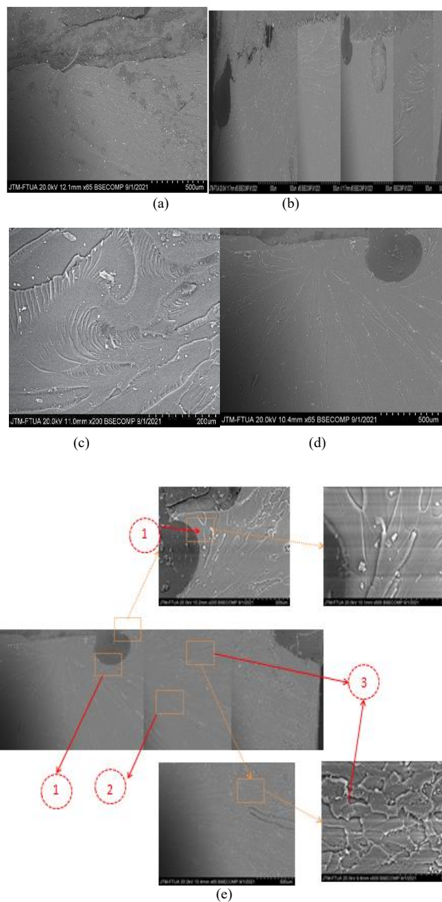
Figure 3: SEM tensile fracture surface of (a) UP 100%, (b) VE 100% (C-e) UP/VE at 40 wt. %
