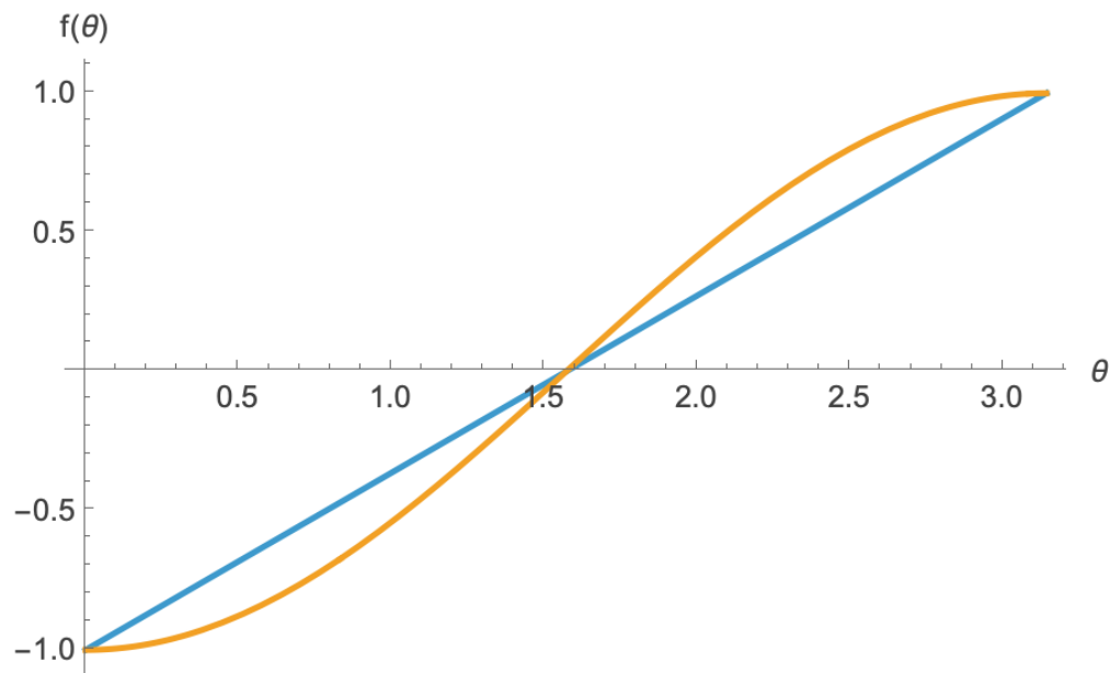
Figure 1: \frac{2\theta}{\pi} - 1 (blue), -\cos(\theta) (orange)
