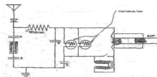
Figure 4: T. H. Moray Radiant Energy Device Schematic
