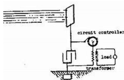
Figure 3: Nikola Tesla Radiant Energy Device Schematic
