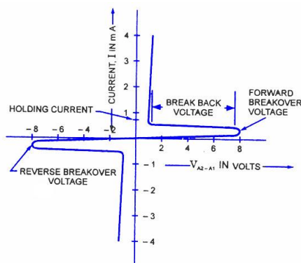
Figure 1. Sidac I-V Discharge Curve
