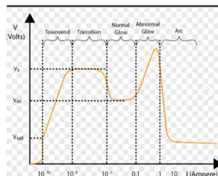
Figure 2. Cold Cathode Tube I-V Discharge Curve
