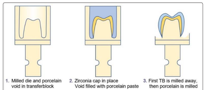
Figure 3: PRIMERO Lab System (DENTALXS.COM, Hoorn, The Netherlands)
