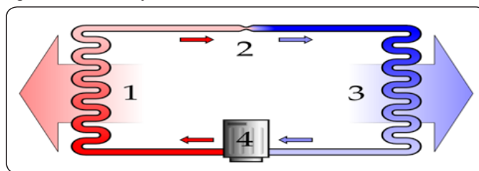
Figure 1: Diagram of a phase change heat pump: 1) condenser coil 2) expansion valve 3) evaporator coil and 4) compressor.
