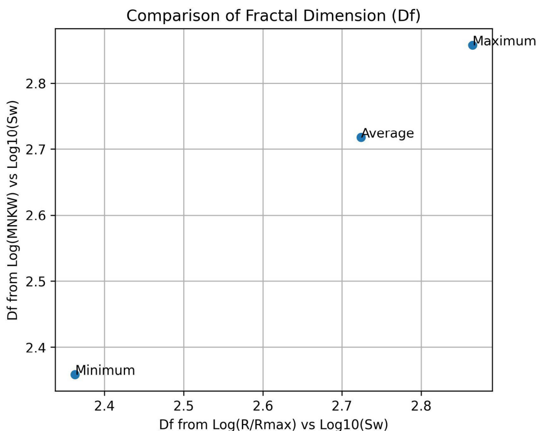
Figure 1: Comparison of Fractal Dimensions (Df) Derived from the \text{Log}(R/R_{\text{max}}) and MNKW Methods for Representative Samples
