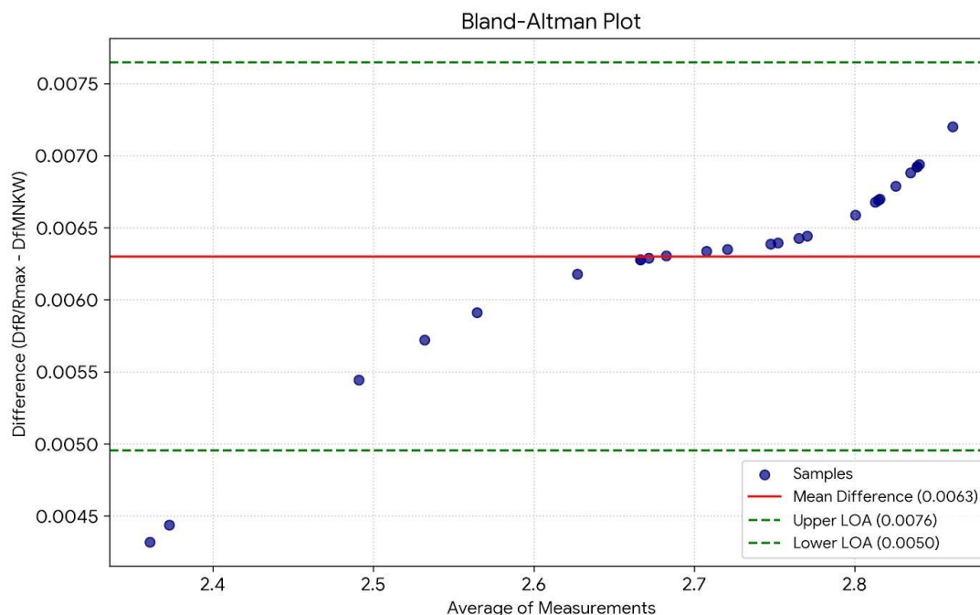
Figure 3: Bland–Altman Plot Showing Bias and Limits of Agreement Between the Two Methods
