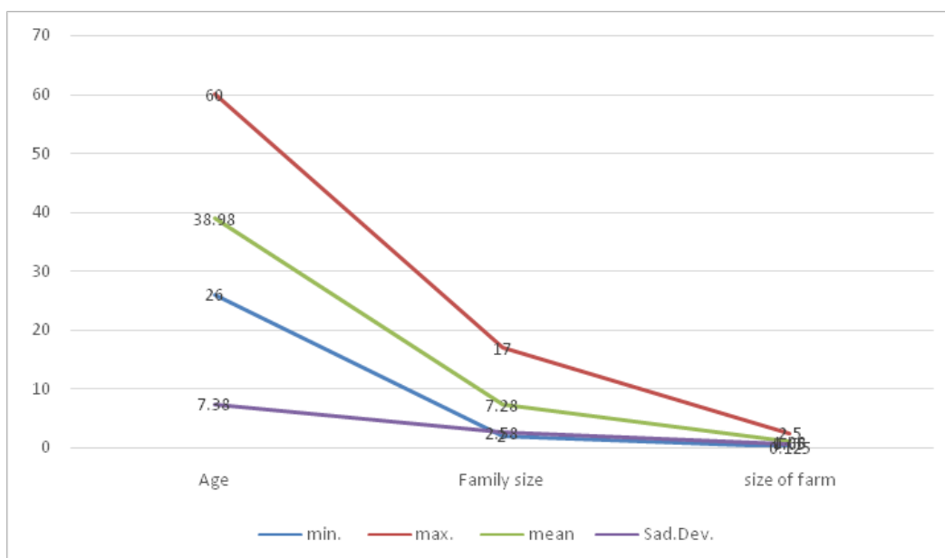
Figure 2: Continuous Variables Description
