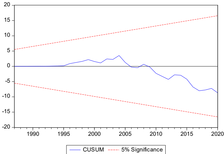
Figure 1: CUSUM Test
