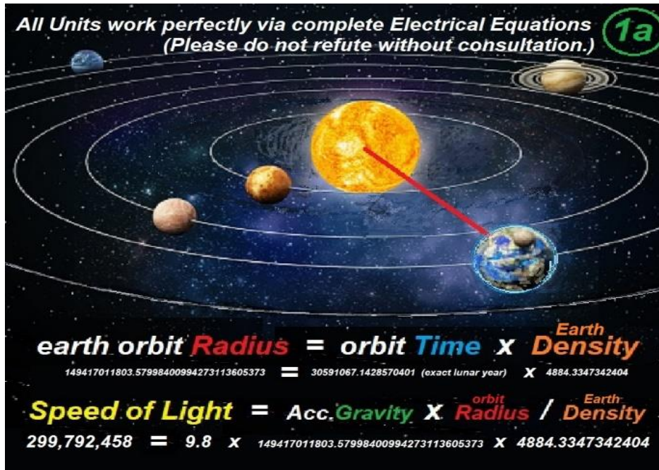
Figure 1a: Earth Orbit Radius.
