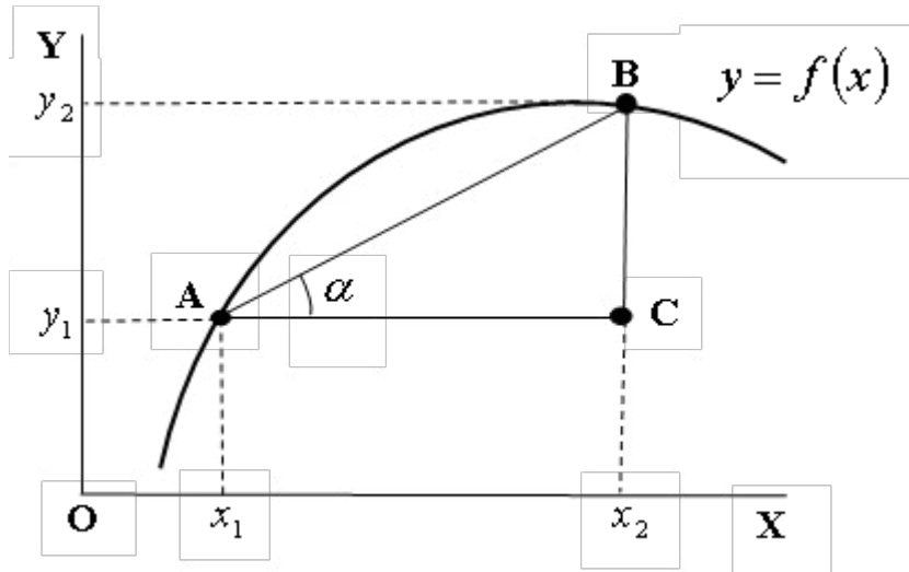
Figure 2. Material system “Segment of the line y = f(x) + right-angled triangle \Delta ABC ” in the Cartesian coordinate system XOY . The \overline{AB} secant is the hypotenuse of the right-angled triangle \Delta ABC . Quantities x_1, x_2, y_1, y_2, are the abscissas and ordinates of the points A, B, C, respectively.
