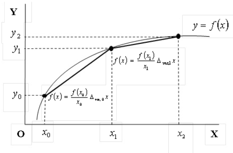
Figure 1. Geometric interpretation of proportion. The broken line, obtained using the method of proportion, approximates the graph of the function y = f(x) . The quantities f(x_1) = \frac{f(x_0)}{x_0} \Delta_{\text{var},0} x and f(x_2) = \frac{f(x_1)}{x_1} \Delta_{\text{var},1} x determine the positions of the vertices of the broken line in the coordinate system XOY .
