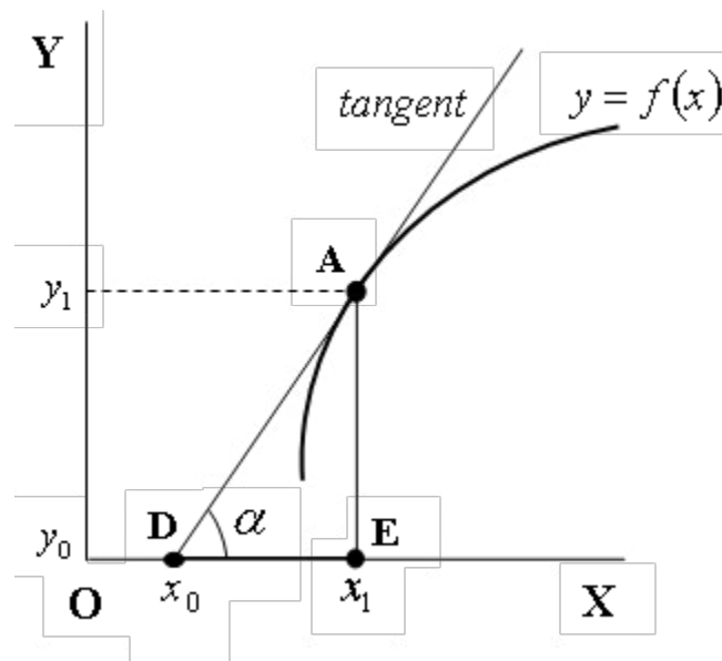
Figure 3: Material system “Segment of line y = f(x) + right-angled triangle \triangle DAE ” in the Cartesian coordinate system XOY . The tangent DA is the hypotenuse of the right-angled triangle \triangle DAE . The constants x_0, x_1, y_0, y_1 are the abscissas and ordinates of the points D, A, E . The quantities \Delta x_{1,0} \equiv x_1 - x_0 \neq 0 and \Delta y_{1,0} \equiv y_1 - y_0 \neq 0 determine the lengths of the legs of the triangle \triangle DAE .
