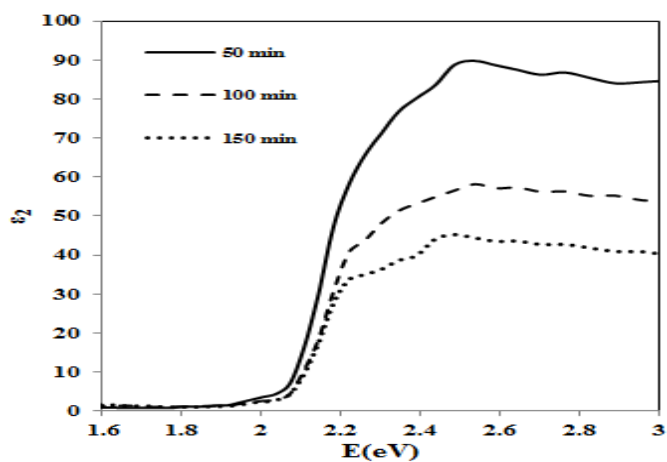
Figure 7: The Imaginary Part of Dielectric Constant of Mercury Sulfide Layers Produced by CBD Method at Different Deposition Times
