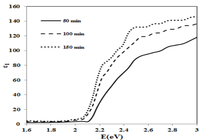
Figure 6: The Real Part of Dielectric Constant of Mercury Sulfide Layers Produced by CBD Method at Different Deposition Times
