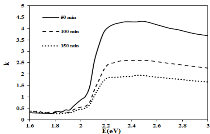
Figure 5: The Imaginary Part of Refractive Index of Mercury Sulfide Layers Produced by CBD Method at Different Deposition Times
