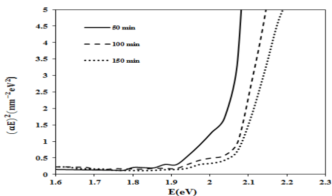
Figure 11: The Values of Band Gap Energy of Mercury Sulfide Layers Produced by CBD Method at Different Deposition Times
