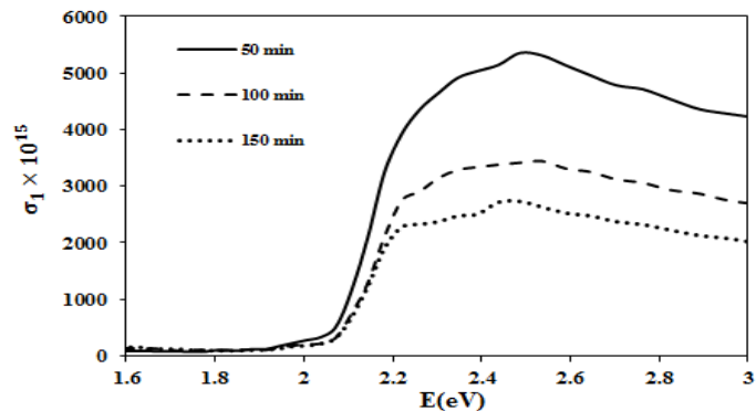
Figure 8: The Real Part of Conductivity Index of Mercury Sulfide Layers Produced by CBD Method at Different Deposition Times
