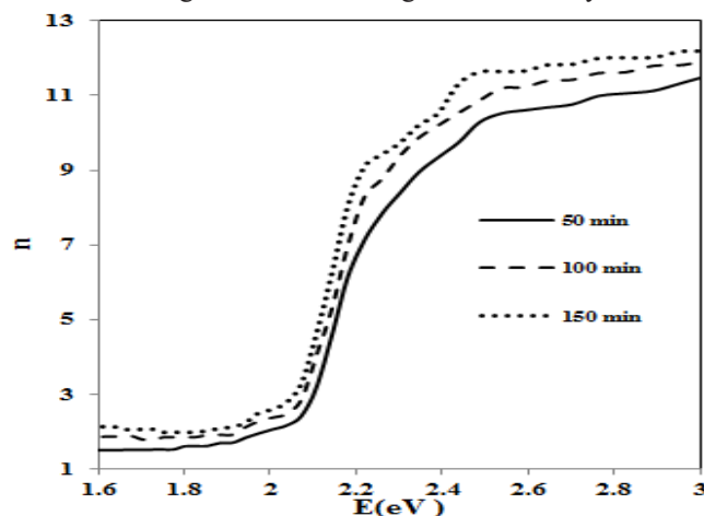
Figure 4: The Real Part of Refractive Index of Mercury Sulfide Layers Produced by CBD Method at Different Deposition Times
