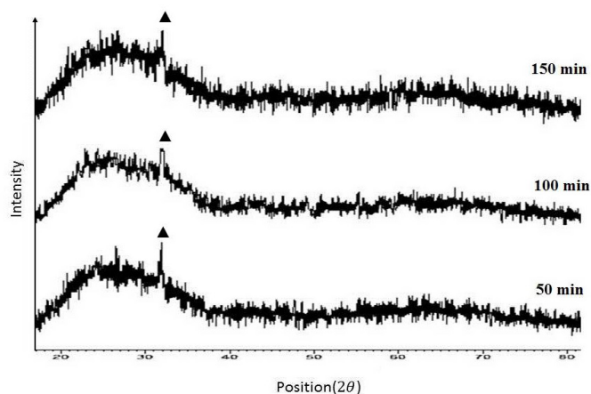
Figure 1: The XRD Spectra of Mercury Sulfide Layers Produced by CBD Method at Different Deposition Times
