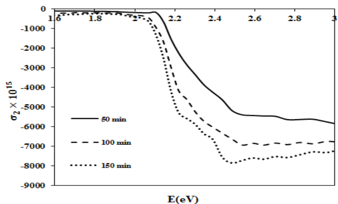
Figure 9: The Imaginary Part of Conductivity Index of Mercury Sulfide Layers Produced by CBD Method at Different Deposition Times
