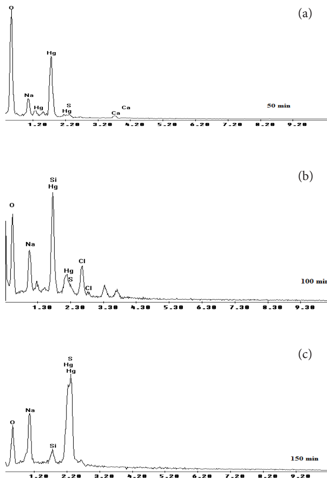
Figure 2: The EDAX Images of Mercury Sulfide Layers Produced by CBD Method at Different Deposition Times
