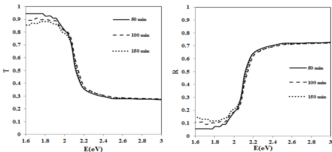
Figure 3: The A) Transmittance and B) Reflectance of Mercury Sulfide Layers Produced by CBD Method at Different Deposition Times
