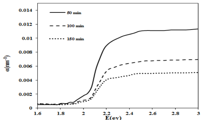
Figure 10: The Absorption Coefficient of Mercury Sulfide Layers Produced by CBD Method at Different Deposition Times
