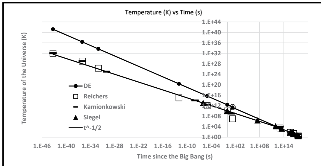
Figure 1: Demonstrating the Difference Between the Dark Energy Theory and the Current Big Bang Theory
