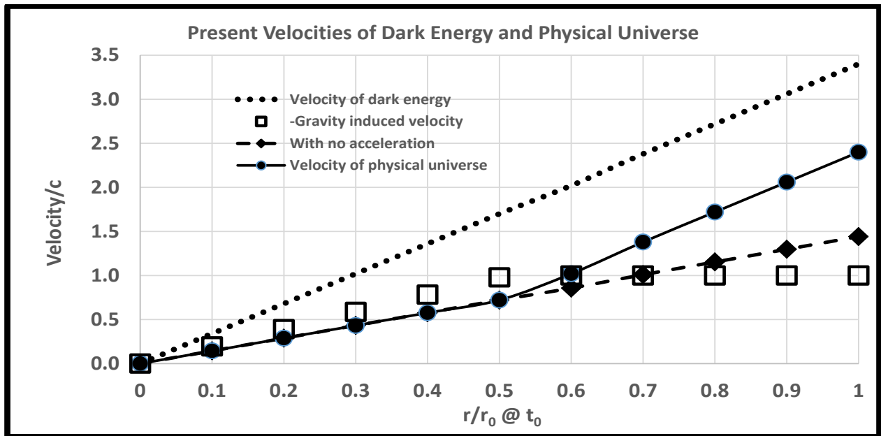
Figure 2: Relative Expansion Rates of Dark Energy and Matter Showing the Effect of Maximum Recession c
