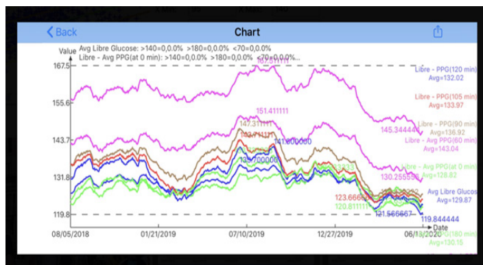
Figure 9: 8 time-series PPG curves
