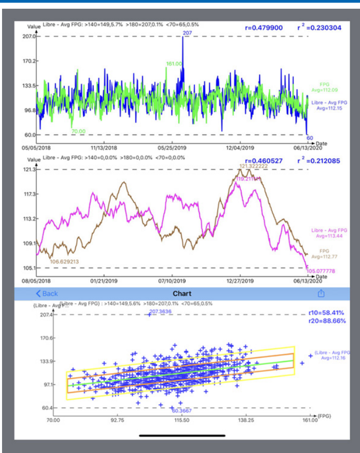
Figure 4: Time-series and spatial analysis results of FPG
