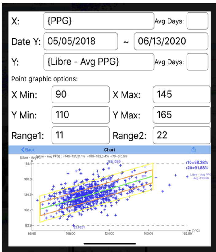
Figure 6: Spatial analysis detailed data of daily PPG
