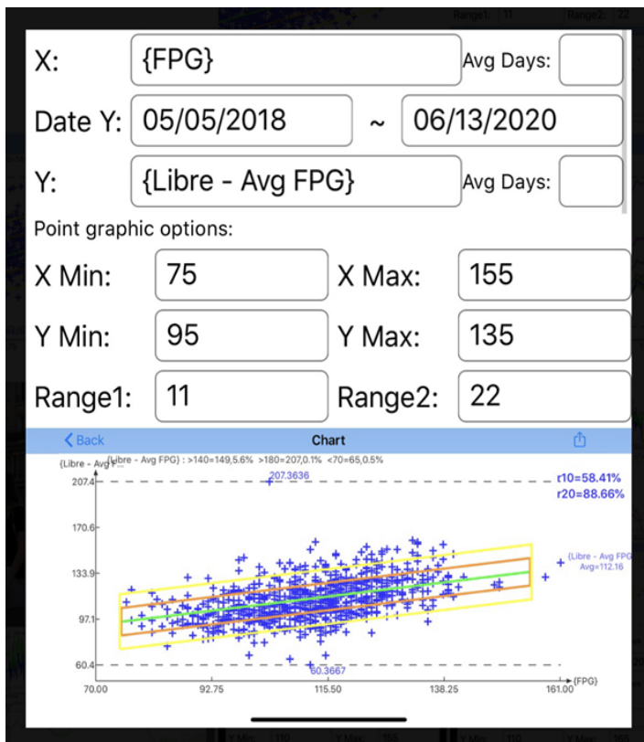
Figure 7: Spatial analysis detailed data of daily FPG
