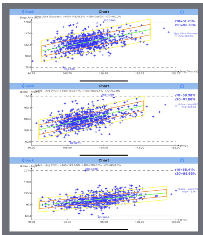
Figure 8: Spatial analysis results comparison of three gluceses
