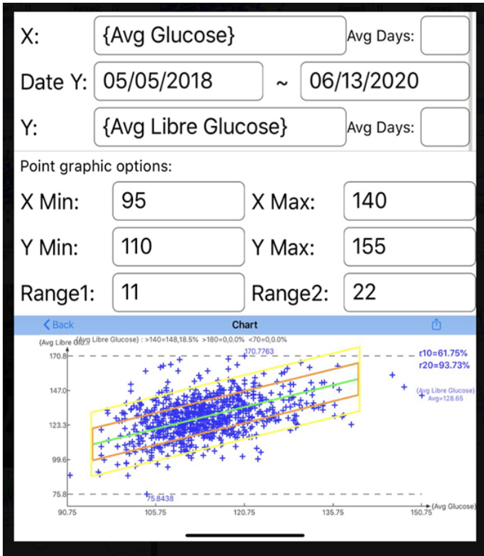
Figure 5: Spatial analysis detailed data of daily glucose
