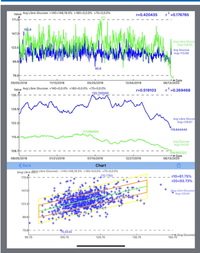
Figure 2: Time-series and spatial analysis results of daily glucose
