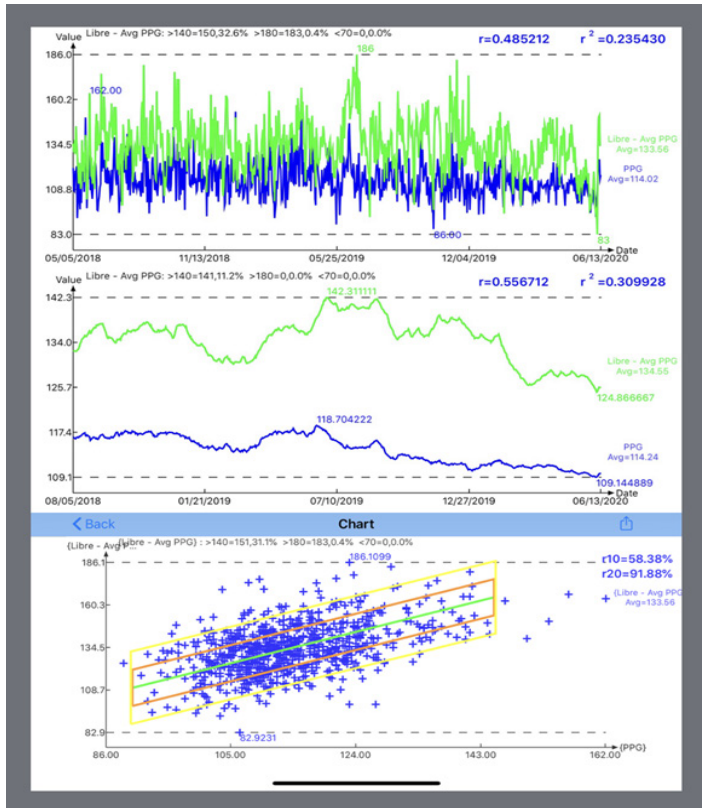
Figure 3: Time-series and spatial analysis results of PPG
