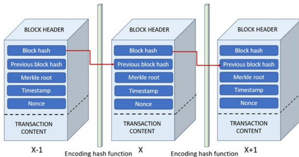
Figure 1: Block structure in a blockchain
