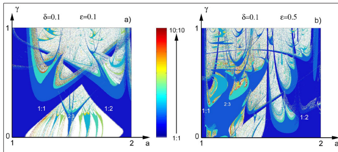
Figure 6: Phase capture areas of a system of oscillators with two-way coupling ( \delta = 0, 1 ): (a) \varepsilon = 0, 1 ; (b) \varepsilon = 0, 5 .
