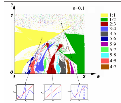
Figure 4: Areas of stable phase captures for piecewise linear mapping of a circle (2) with a PRC of the form (6) taking into account the mutual influence of oscillators.
