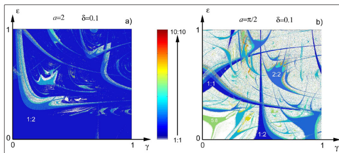
Figure 7: Phase captures in the stimulus amplitude space ( \delta = 0, 1 ): (a) a = 2 ; (b) a = \pi/2 .
