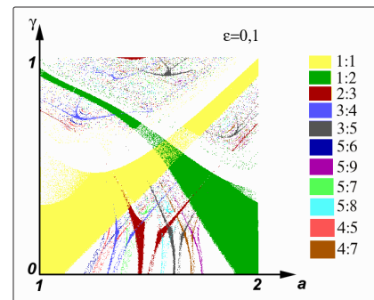
Figure 5: Phase diagram of the sine curve (7) taking into account the mutual influence of oscillators.
