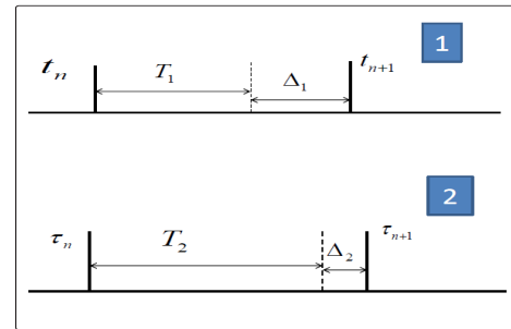
Figure 3: The scheme of construction of the model describing the system of two interacting nonlinear oscillators
