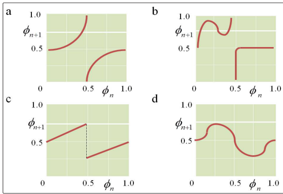
Figure 1: Different types of circle maps: (a) reversible, topological degree 1; (b) irreversible, topological degree 1; (c) piecewise continuous; (d) topological degree 0.
