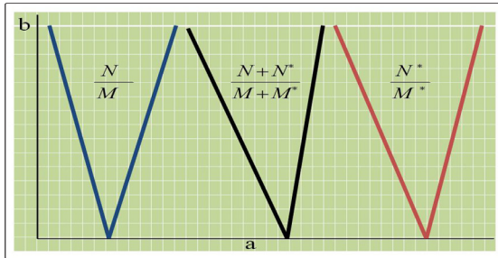
Figure 2: Schematic diagram of Arnold tongues. In shaded areas there is a steady phase capture. There are always other zones between any two capture zones.
