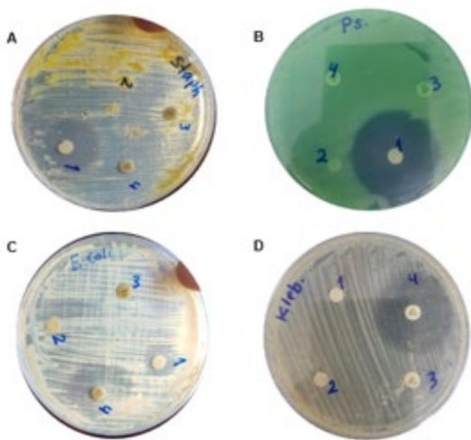
Figure 2: Antimicrobial activity of (1) probiotic Lactobacillus strains supernatant, (2) BHIB (negative control), (3) Ampicillin, and (4) Gentamicin against different test pathogens A Staphylococcus aureus , B Pseudomonas aeruginosa , C Escherichia coli , and D Klebsiella pneumoniae by the disk diffusion method.
