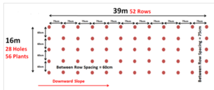
Figure 1: Layout of a Pfumvudza plot
