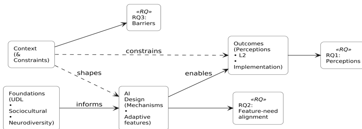
Figure 1: Integrative Theoretical Framework for AI for Neurodiverse L2 Learners
