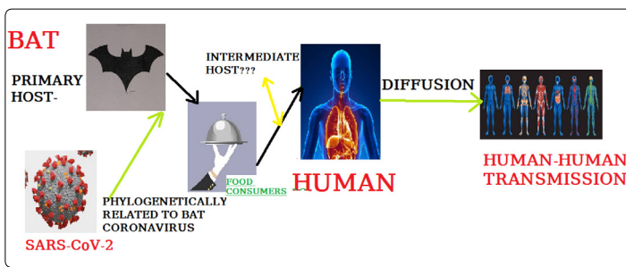
Figure 1: SARS-COV-2 Transmission [2].
