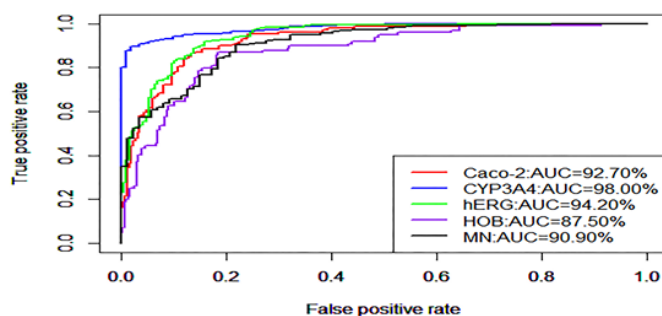
(c) GBM-ROC
