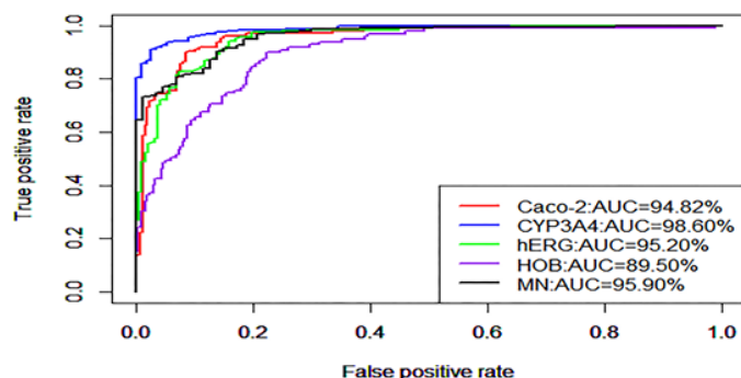
(a) XGBoost-ROC
