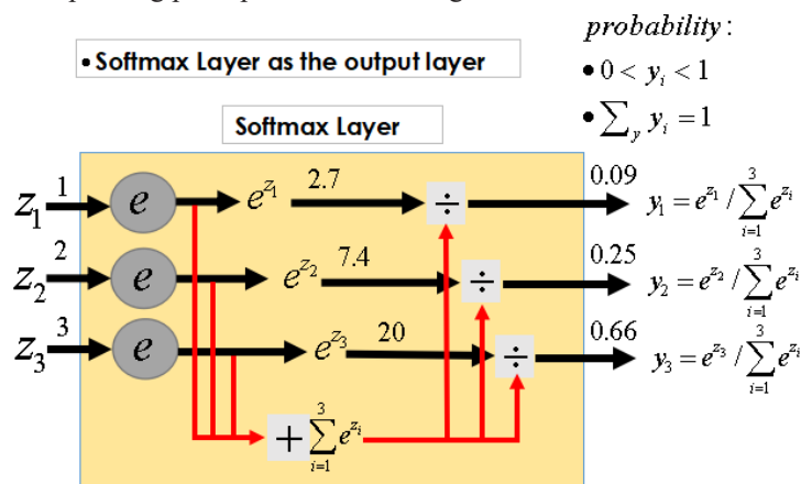
Figure 2: Principle of Softmax Function
