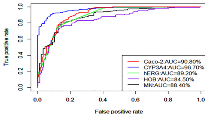
(b) One-layer BPNNet-ROC
