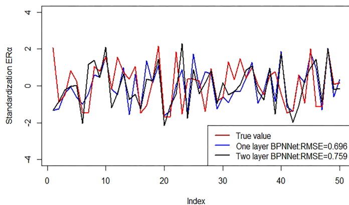
Figure 4: The Predict of Adam-BPNNet
