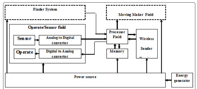
Figure 4: Internal structure of operate/sensor node [19]
