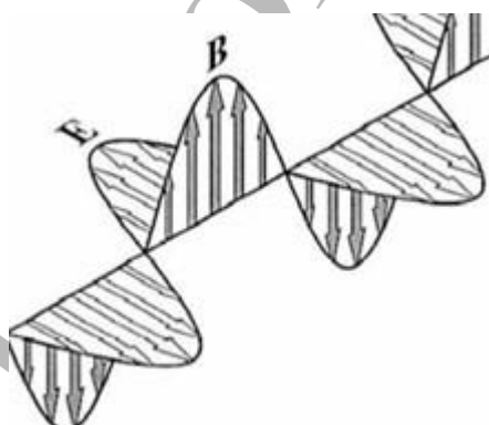
Figure 1: B. Light is a wave composed of oscillating electric ( \vec{E} ) and magnetic ( \vec{B} ) field vectors that give the appearance of dumbbell shapes. This dumbbell-like shape when split into individual wave sections (photons) can give the appearance of either a particle or a wave. This splitting apart can be as small as Planks constant or one wavelength. Wikipedia Creative Commons.
