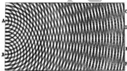
Figure 10: Water Ripple Tank Interference
