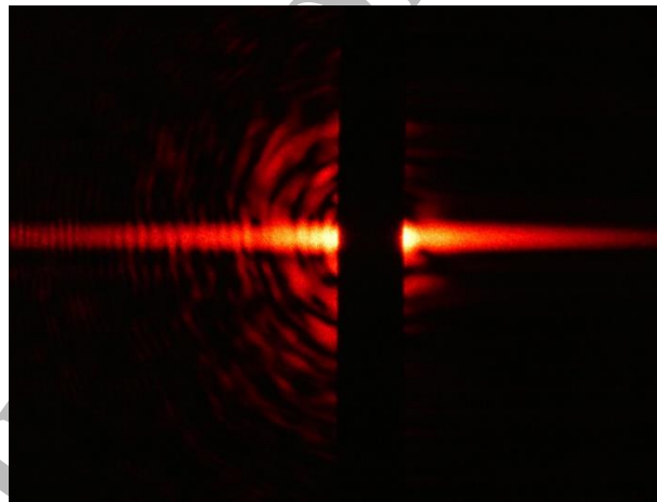
Figure 6: The Photons have Reflected to the Left and Diffracted to the Right. The line to the left of center is also considered diffraction. Note: The center bright spot was blocked off to avoid over exposure. Note: The human eye is unable to determine intensity differences correctly. https://www.telescope-optics.net/eye_intensity_response.htm
