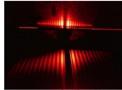
Strands of Light Figure 14
