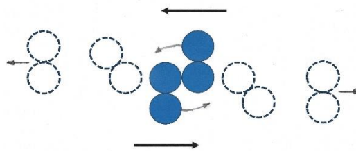
Figure 3: Similar to (Figure 2). The collision of two off-center dumbbells in the absence of a barrier. How two opposing beams of light can appear to pass directly through one another.
