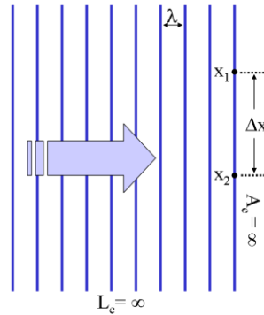
Figure 17: A Plane Wave with Infinite Coherence Length
