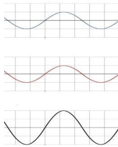
Figure 19: The Addition of Water Waves
