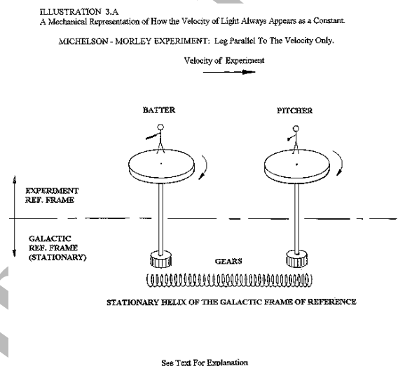
Figure 21: Mechanical Representation of How the Velocity of Light Always Appears as a Constant
