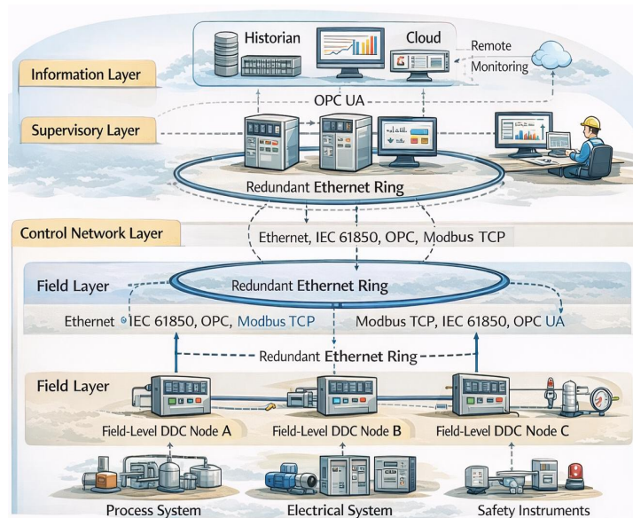
Figure 3: Proposed DDC-based Integrated Electrical and Instrumentation Control System Architecture Illustrating Distributed Field-level Autonomy, Subsystem Interoperability, and System-of-Systems Integration
